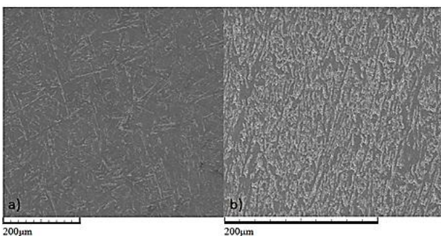
Fig. 4 – Distribution of martensite phase in microstructure of alloy: (a) E_0 ; (b) E_3
