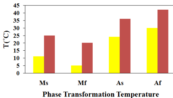
Fig. 7 – Comparison of phase transformation temperatures of E_0 (yellow columns) and E_3 (red columns)
