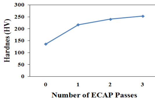
Fig. 8 – Microhardness values of the samples
