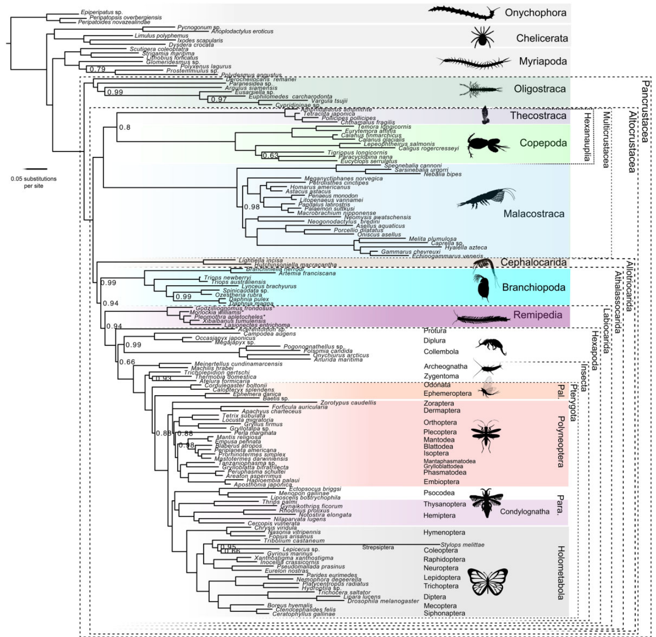
Fig. 2. —Phylogenetic tree derived from the CAT-GTR+G analysis of the Matrix A recoded version of the data under Dayhoff-6. Newly sequenced transcriptomes are marked with an asterisk. Burnin = 2,500, Total Cycles = 10,000, subsampling frequency = 10, Maxdiff = 0.22, Minimal effective size = 64. Support values represent posterior probabilities and only those < 1 are shown. Para., Paraneoptera; Pal., Paleoptera.
