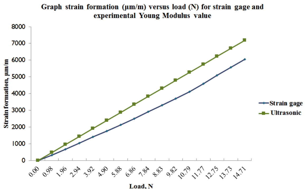
Fig. 5 Results obtained using a strain gage and an ultrasonic system
