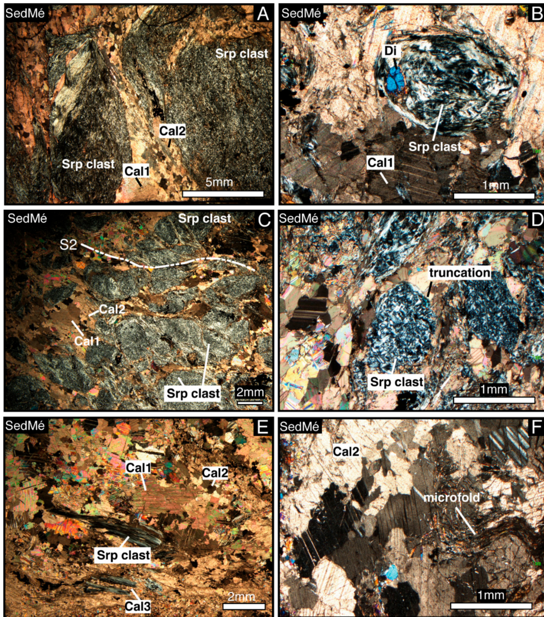
Figure 10. Photomicrographs illustrating the main microstructural features of SedMé. All pictures are taken in crossed-polarized light. Mineral abbreviations after [104]. (A) Millimeter- to centimeter-sized ultramafic (serpentinite) clasts embedded in a Cb-rich matrix. Clasts have sub-rounded to elongated shapes. Their boundaries are either truncated or transposed near the contact with the Cb-rich matrix. Clasts on the left show an internal foliation marked by the shape preferred orientation (SPO) of Srp. Foliation is crenulated without the development of a differentiated cleavage. Calcite porphyroblasts (Cal1) and neoblasts (Cal2) are visible in the carbonate-rich matrix. (B) Serpentinite clast with Di grain (see text). The clast internal foliation is folded and truncated along the clast margins without drag into the matrix foliation (probably enhanced by dissolution/precipitation). (C) Foliated type of SedMé. Foliation ( S_2 ) is defined by SPO of ultramafic clasts or clast aggregates and by carbonate (Cal2) ribbons. Microboudinage of clasts is also recognizable. (D) Ultramafic clasts preserving internal relict (or recrystallized) mesh-texture of serpentine. Clasts show either transposed or truncated edges. Truncation is probably enhanced by dissolution/precipitation. (E) Matrix-supported type of SedMé characterized by mm- to cm-sized ultramafic clasts diffusively transposed within the matrix consisting of isotropic or weakly foliated fabric. (F) Relic of S_1 foliation marked by microfolded layers composed of Cal1 and Amp1 in isotropic types of SedMé.
