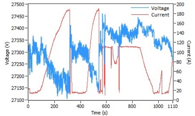
Fig. 3. r.m.s value of voltage and current at a pantograph level
