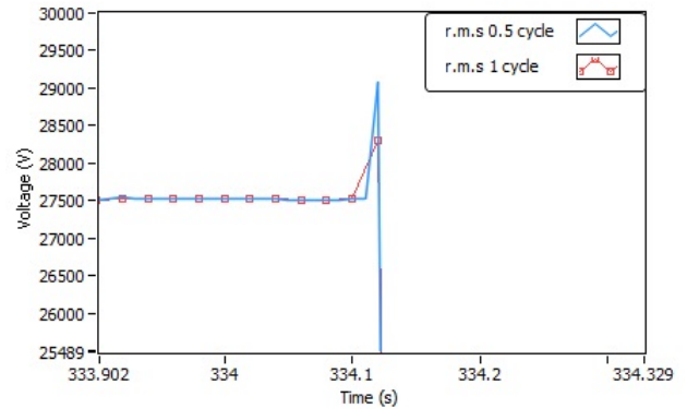
Fig. 13. Voltage swell measured as r.m.s value over 1 cycle and half cycle
