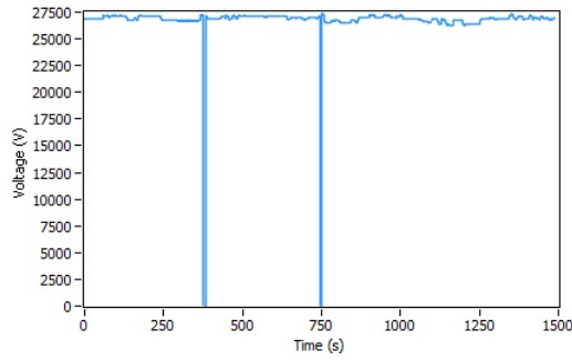
Fig. 7. Supply voltage interruptions registered in segment 2 of the network
