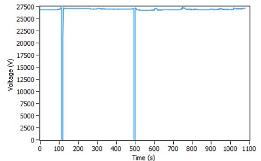
Fig. 6. Supply voltage interruptions registered in segment 1 of the network
