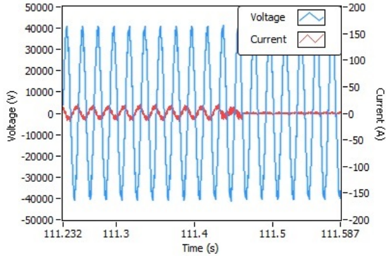
Fig. 8. Voltage and current before the interruption 1 in the segment 1
