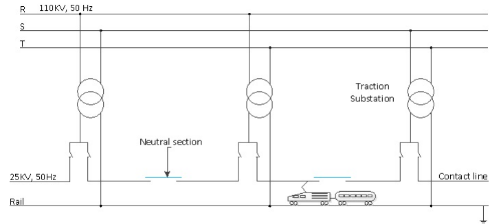
Fig. 5. Power supply network example in AC traction systems
