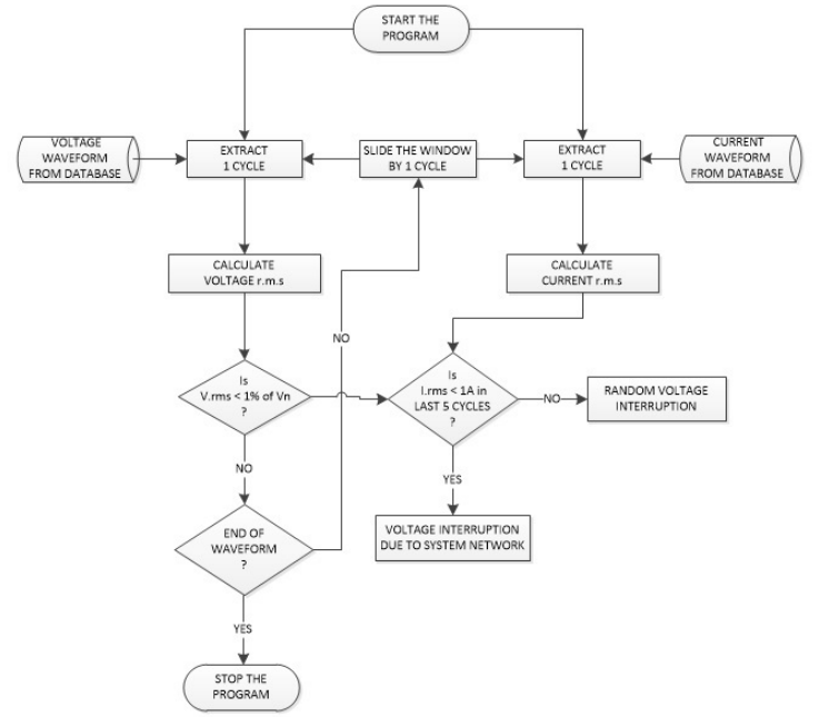
Fig. 10. Flowchart of the proposed measurement technique for classification of voltage interruptions
