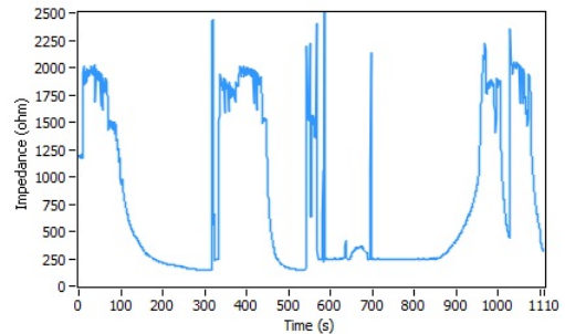
Fig. 4. Dynamic impedance of the traction unit
