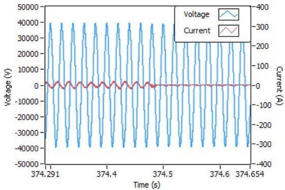
Fig. 9. Voltage and current before the interruption 1 in the segment 2
