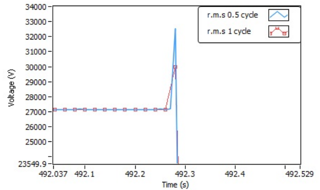
Fig. 12. Voltage swell measured as r.m.s value over 1 cycle and half cycle
