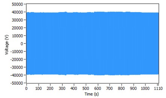
Fig. 1. Instantaneous voltage at the pantograph
