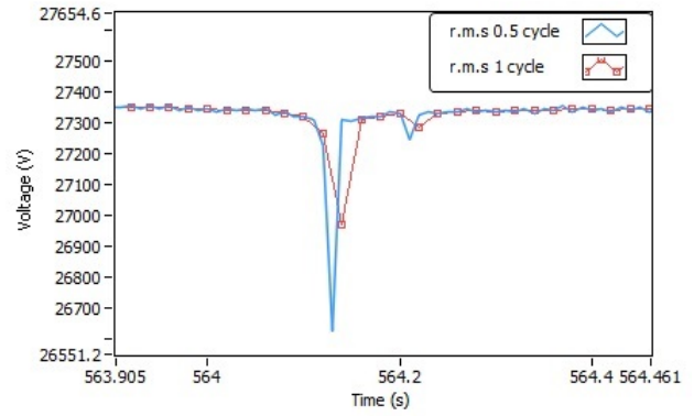
Fig. 11. Voltage dip measured as r.m.s value over 1 cycle and half cycle
