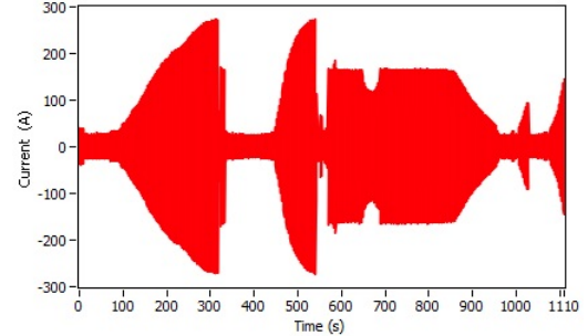
Fig. 2. Instantaneous current at the pantograph
