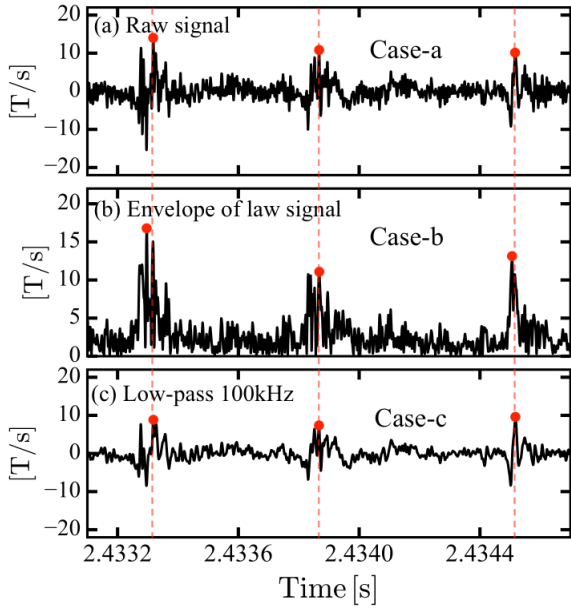
Fig.2: The threshold method is performed for 3 different proceeded signals of dB/dt bursts. (a) Raw signal, (b) envelope of the raw signal, and (c) low-pass 100 kHz signal are used and named as Case-a, Case-b and Case-c, respectively. Thresholds are defined as 10, 10 and 7 T/s, respectively. The red points indicate the clocks for each case, and red dashed line shows the timing of clocks of Case-a.
