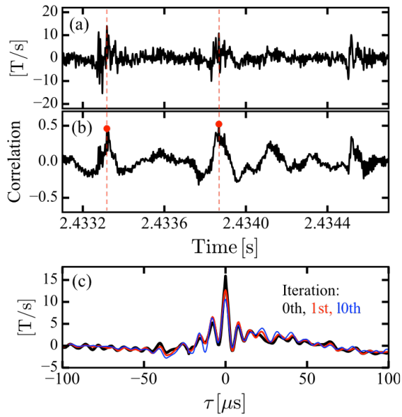
Fig.4: The procedure of the template method is shown. (a) Raw signal of dB/dt and (b) cross correlation between raw signal and initial template where the red point indicates the clocks. (c) initial/0 th iterated template (black), 1 st iterated template (red) and converged, 10th iterated template (blue).
