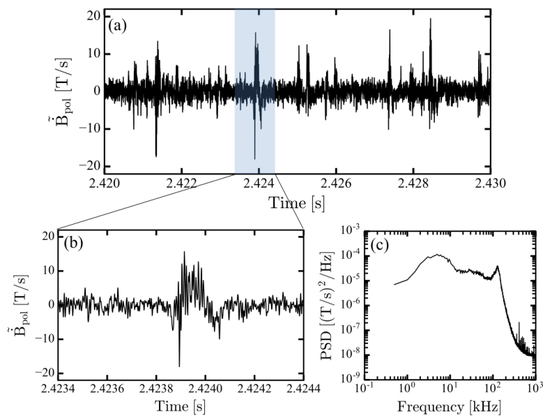
Fig.1: (a) Raw signal of dB/dt fluctuations measured by Mirnov coil. (b) Enlarged view of the burst. (c) Power spectrum of the dB/dt fluctuations.
