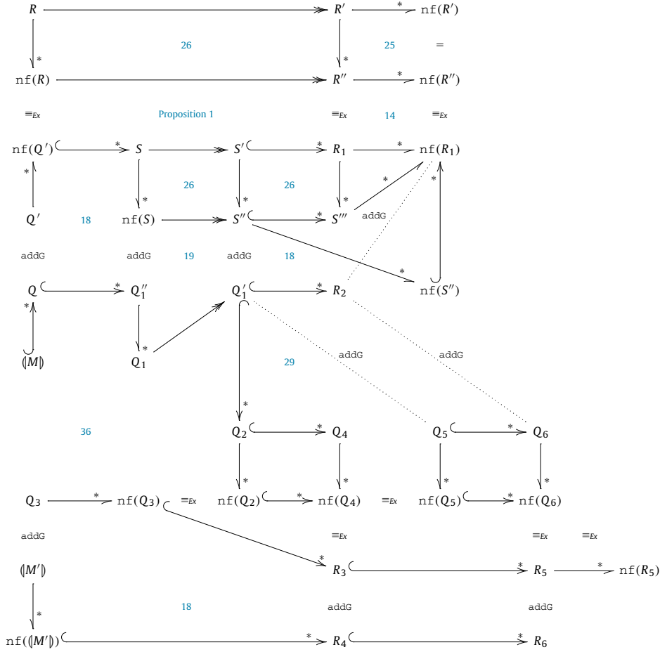
Fig. 15. Proof schema of Theorem 3, challenge R \rightarrow R' .
