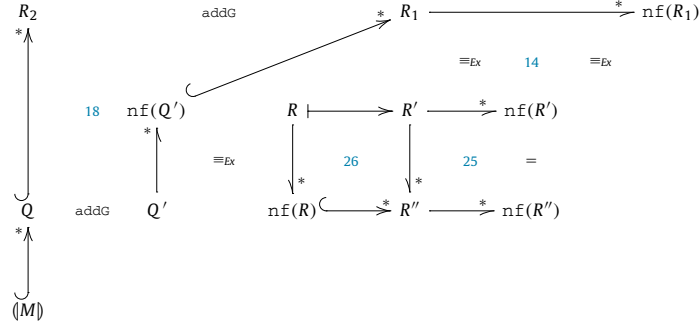
Fig. 14. Proof schema of Theorem 3, challenge R \mapsto R' .
