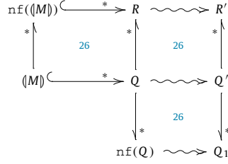
Fig. 12. Proof schema of the first part of Lemma 37.
