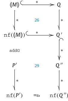
Fig. C.18. Proof schema of Lemma 30 (numbers refer to Lemmas).
