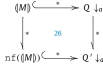
Fig. C.19. Proof schema of Lemma 63 (numbers refer to Lemmas).
