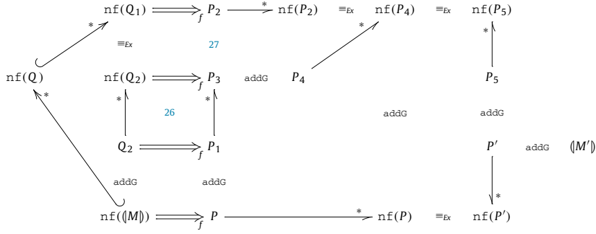
Fig. 13. Proof schema of Theorem 3, challenge M \rightarrow M' .
