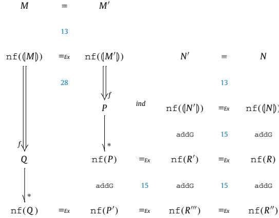
Fig. 9. Proof schema of Theorem 4, case Equiv (numbers refer to Lemmas).
