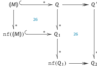
Fig. 10. Proof schema of the first part of Lemma 36.
