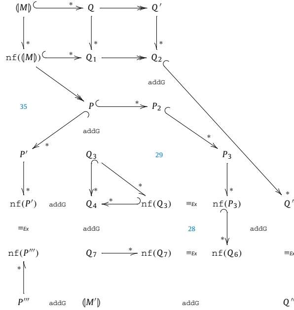
Fig. 11. Proof schema of the last part of Lemma 36.
