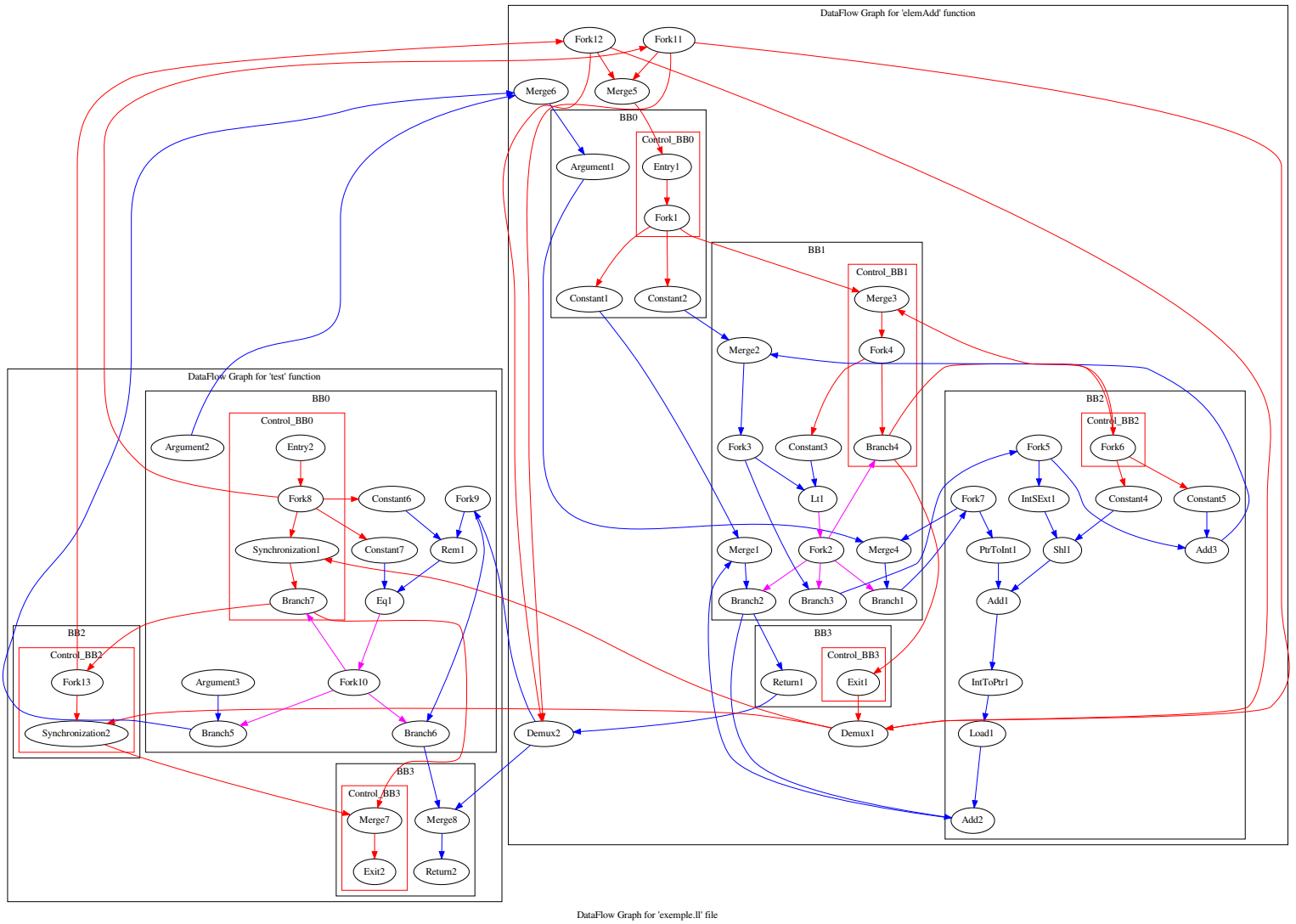
Figure 27: Example 1 - Data flow graph (Source: own compilation)
