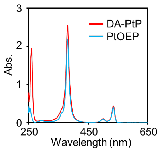
Figure S3. (a) UV-vis absorption spectra of DA-PtP and PtOEP in DMSO ( 5 \mu\text{M} ).
