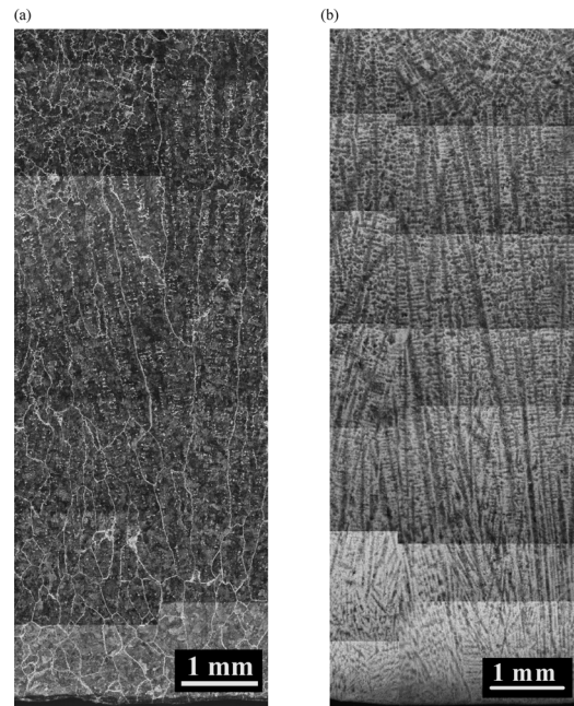
Fig. 2. Optical micrographs on the transverse section showing (a) \gamma -grain and (b) \delta -dendrite structures in as-cast sample without titanium addition. The top and the bottom of each micrograph correspond to the center and the surface of the ingot, respectively.
