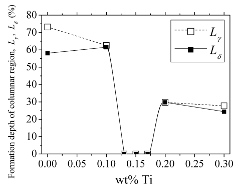
Fig. 8. Effect of Ti addition on formation depth of \gamma ( L_\gamma ) and \delta ( L_\delta ) columnar regions.
