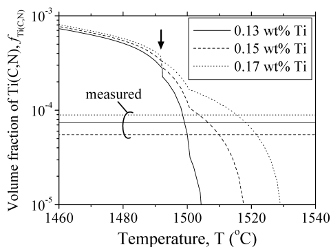
Fig. 11. Calculated volume fractions of Ti(C,N) during equilibrium solidifications. Three horizontal lines represent measured volume fractions of faceted Ti(C,N) particles. The peritectic reaction temperature is indicated by the arrow.
