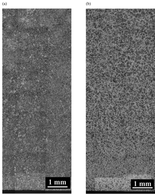
Fig. 4. Optical micrographs on the transverse section showing (a) \gamma -grain and (b) \delta -dendrite structures in as-cast sample with addition of 0.15 wt% Ti. The top and the bottom of the each micrograph correspond to the center and the surface of the ingot, respectively.
