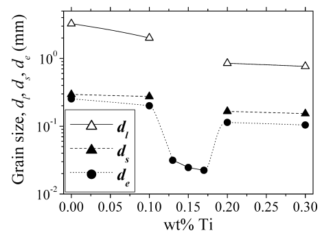
Fig. 3. Effect of Ti addition on \gamma grain sizes. d_l is \gamma -grain size across long axis and d_s is \gamma -grain size across short axis in the columnar region, while d_e denotes the equiaxed grain size.
