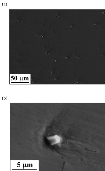
Fig. 7. (a) SEM image of Ti(C,N) particles in as-cast sample with addition of 0.15 wt% Ti. (b) Enlargement of Ti(C,N) particle with faceted shape.
