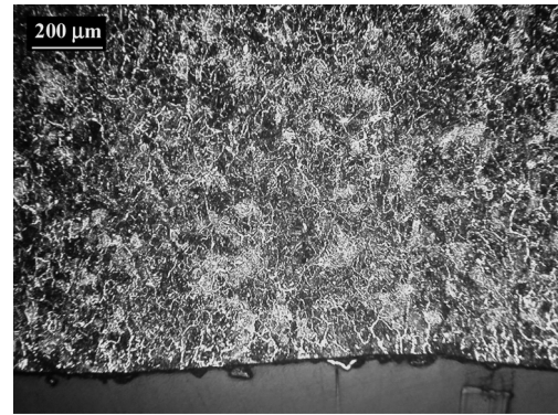
Fig. 5. Enlargement of \gamma -austenite structure in as-cast sample with addition of 0.15 wt% Ti. The bottom of micrograph corresponds to the surface of the ingot.
