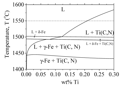
Fig. 6. Calculated phase diagram of Fe–0.435wt%C–0.0052 wt%N–Ti system based on the thermodynamic assessment reported by Lee. 15) The dashed line represents the holding temperature, 1550°C, before the casting operation.
