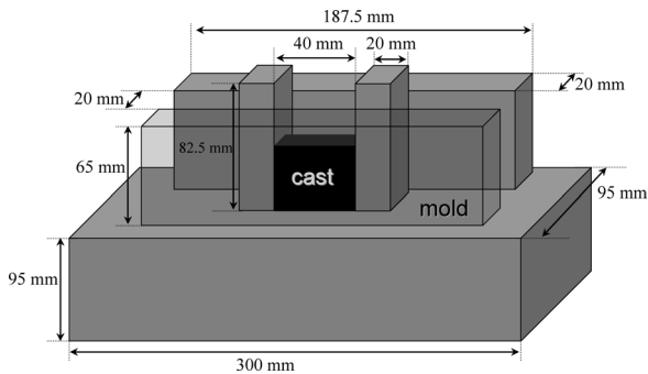
Fig. 1. Schematic illustration of the steel mold employed in the casting experiment.
