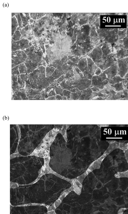
Fig. 10. (a) Equiaxed \gamma structure in as-cast sample with 0.15 wt% Ti. (b) Equiaxed \gamma and \delta structures in as-cast sample with 0.15 wt% Ti. Equiaxed \delta -dendrite structure is superimposed on \gamma structure shown in (a).
