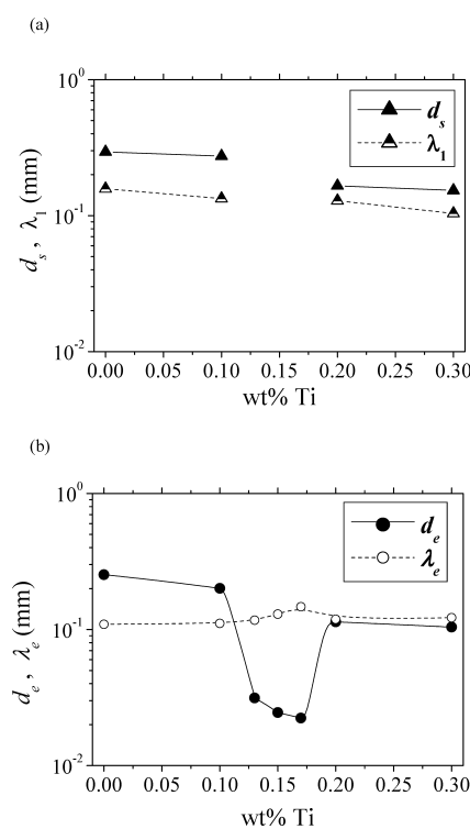
Fig. 9. (a) Dependence of columnar \gamma -grain size across short axis, d_s , and primary arm spacing of columnar \delta -dendrites, \lambda_1 , on titanium addition. (b) Dependence of equiaxed \gamma -grain size, d_e , and center-to-center spacing of equiaxed \delta -dendrites, \lambda_e , on titanium addition.
