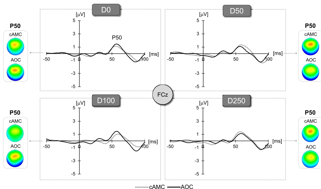
Fig. 2. The P50 response to self-generated and externally generated tones at each delay (D0, D50, D100, D250).
