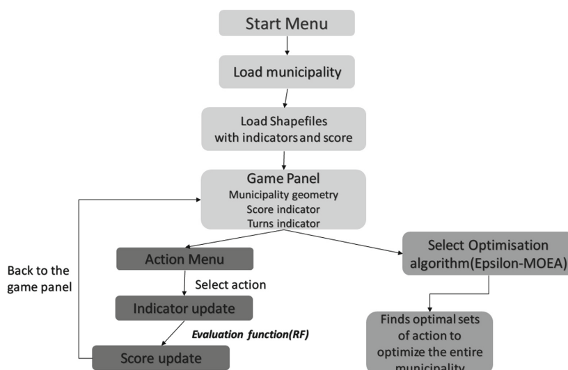
Fig. 6. Pipeline of the simulation
