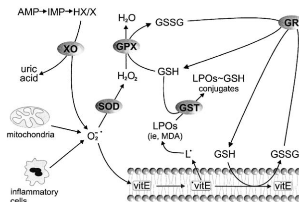
Figure 1 A schematic representation of antioxidants and ROS formation. AMP: adenosine monophosphate; IMP: inosine monophosphate; XO: xanthine oxidase; HX: hypoxanthine; X: xanthine; SOD: superoxide dismutase; GPX: glutathione peroxidase; GSH: reduced glutathione; GSSG: oxidized glutathione; GR: glutathione reductase; GST: glutathione S-transferase; L: lipid radical; LPOs: lipid peroxidation products; MDA: malondialdehyde; vitE: vitamin E.
