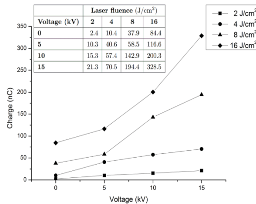
Figure 5: Total extracted charge as a function of the accelerating voltage for different values of the laser fluence
