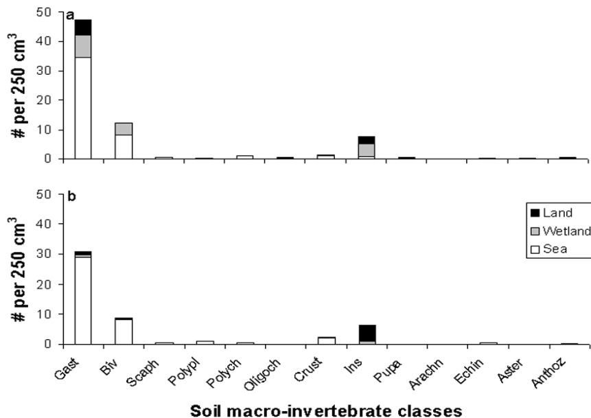
Figure 3. Mean density of substratum macroinvertebrate taxa among sea, wetland and land units of five coastal wetlands (N=5) in: a) spring and b) autumn of 2005. Gast: gasteropoda, Biv: bivalvia, Polyp: polyplacophora, Polych: polychaeta, Oligoch: oligochaeta, Crust: crustacean, Ins: insecta (mature), Pupa: insecta (immature), Arachn: arachnidae, Echin: echinodermata, Aster: asteroidea, Anthoz: anthozoan.
