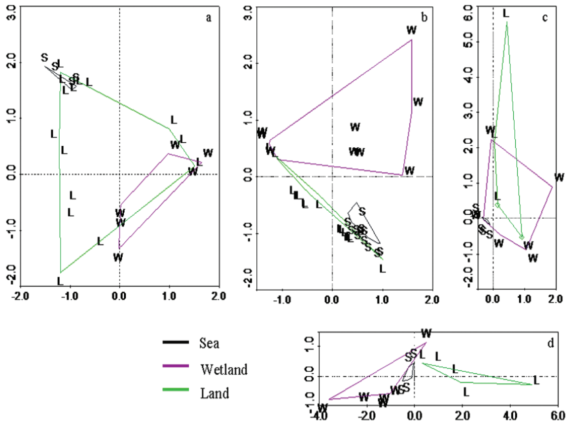
Figure 4 - Samples scatterplots based on areal cover of plant species in spring (a) and autumn (b) and on mean total abundance of substratum macroinvertebrate taxa in (c) spring and (d) autumn. Separation among spatial units (sea, wetland, land) is shown with envelopes enclosing all samples of a particular spatial unit.
