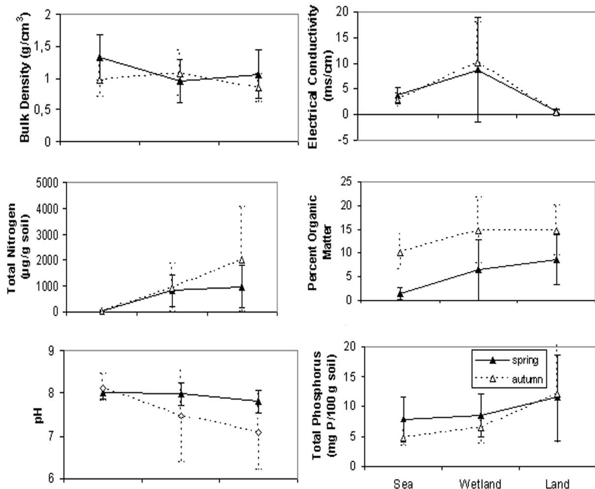
Figure 1 - Spatial variation (mean±stdev) in substratum properties across five coastal wetland systems of Kalloni bay, in spring and autumn of 2005, N=25.
