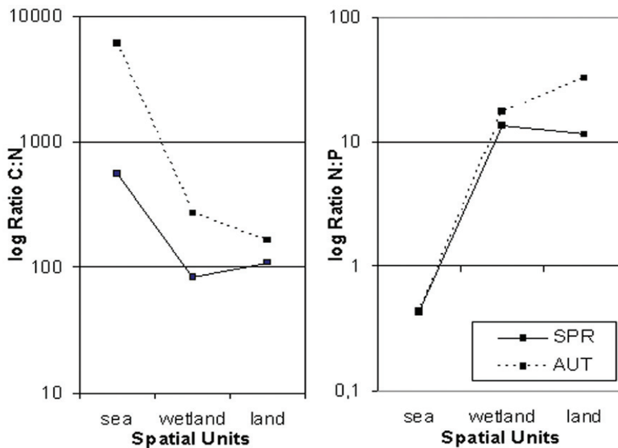
Figure 2 - Spatial and seasonal variation in C:N and N:P ratios of substratum, N=25.
