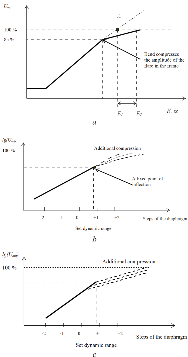
Figure 1 – Electronic methods of dynamic range compression: a – linear compression with the displacement of the point of saturation down; b – nonlinear compression after the inflection point for different contrast; c – options linear compression with the same contrast
