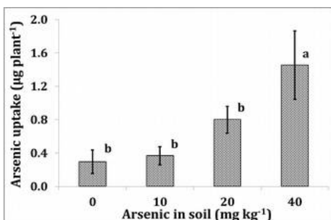
Fig. 2. Arsenic uptake ( \mu\text{g plant}^{-1} ) in plant parts treated with different level of As in growth medium. Different letters above the bars indicate the significant differences ( p=0.05 ). Error bars are the standard deviations ( n=3 ).
