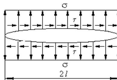
Fig. 9. Action of constant loading on coast of a crack
