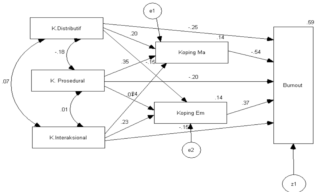
Gambar 1. Full Model Struktural
