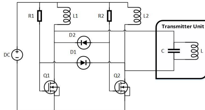
Figure 2. Self- Oscillating PEC circuit
