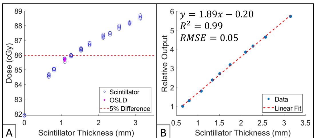
Figure 7. (A) Impact of scintillator thickness on surface dose measured by IC. All data points are normalized to IC reading obtained with no dosimeter present (baseline). 5% from baseline is shown as a dotted red line. IC measurements obtained with scintillators and an OSLD placed upon the IC are shown in hollow blue circles and filled pink dots, respectively. (B) Scintillator light output as a function of thickness. All data points are normalized to the thinnest dosimeter (0.66 mm). Linear fit, as well as corresponding R^2 and RMSE are shown.
