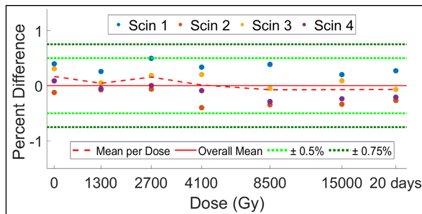
Figure 6. Scintillator output for a group of 4 new scintillators after being exposed to a cumulative dose of 15 000 Gy. Data is presented as percent difference from overall mean of all data collected (solid red line). A verification measurement taken 20 d post-15 000 Gy exposure is also shown. Mean percent difference from overall mean per exposed dose is displayed as a dotted red line. \pm 0.5\% and \pm 1.0\% are in dotted light and dark green lines, respectively.
