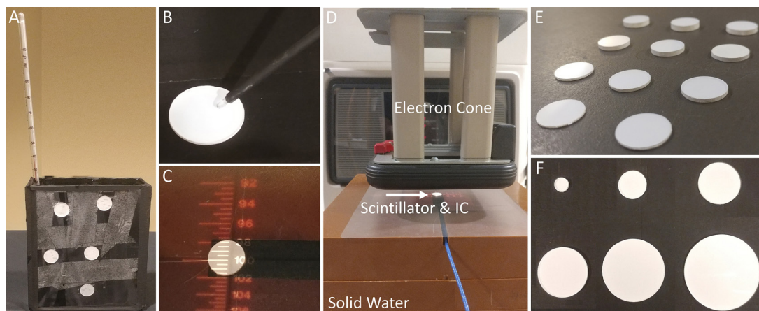
Figure 2. (A) Setup for temperature versus scintillator light output (B) spectrometer fiber optic probe setup (C) scintillator placed on-top of active volume of IC (D) set-up for testing effect of scintillator thickness on surface dose. Solid water, electron cone, and scintillator placed on-top of active volume of IC are labeled (E) scintillators of varying (0.65–3.13 mm) thickness (F) scintillators of varying (5–30 mm) diameters.
