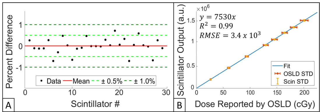
Figure 5. (A) Scintillator-to-scintillator variation for 29 dosimeters. Mean of all percent differences, \pm 0.5\% and \pm 1.0\% are shown red, light green, and dark green, respectively. (B) Scintillator output versus dose reported by OSLD. Linear fit, OSLD STD, and scintillator STD are shown in blue, red and yellow, respectively. Equation for trendline, R^2 , and RMSE are also provided.
