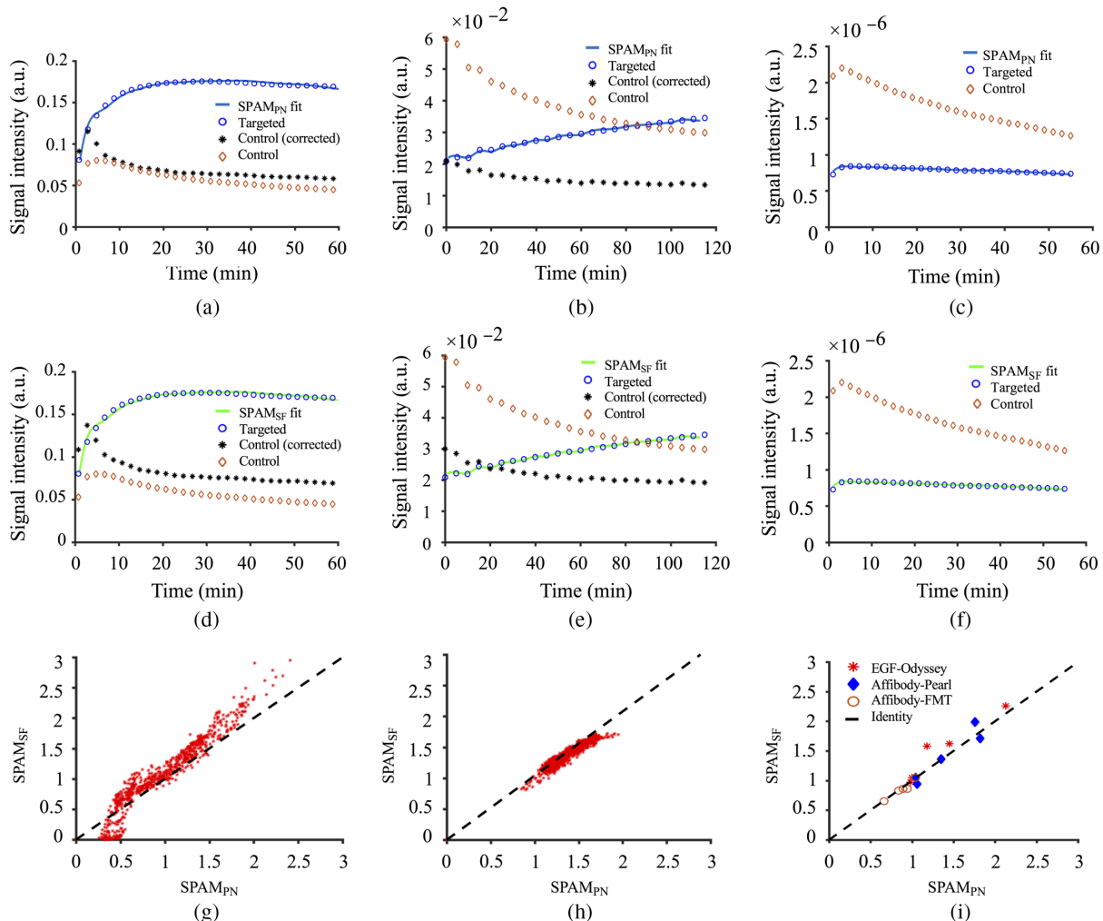
Fig. 5 In vivo experimental results: The linearized pixel-normalization simplified paired agent model SPAM PN in (a) targeted (IR dye 800CW-EGF) and control (IR dye 700DX) imaging agent signal curves measured with the Odyssey System in exposed subcutaneous human glioblastoma (U251) tumors grown in athymic mice, (b) targeted (IR dye 800CW-anti-EGFR-Affibody) and control (IR dye 700DX-negative-control-Affibody) imaging agent signal curves measured with the Pearl System in exposed subcutaneous U251 tumors and (c) targeted (IR dye 800CW-anti-EGFR-Affibody) and control (IR dye 700DX-negative-control-Affibody) imaging agent signal curves measured with an MRI-FMT system from a typical tumor region-of-interest, respectively. Corresponding model fits using the scaling factor SPAM (SPAM SF ) are presented in (d)–(f), respectively. The blue dots represent the targeted imaging agent signal intensity, the orange dots represent the control imaging agent signal intensity before correcting for plasma input function differences, the black dots represent the control imaging agent signal intensity after correcting for plasma input function differences. The solid light blue line represents the SPAM PN fit and the solid green line represents the SPAM SF fit. In (g) and (h) a pixel-by-pixel correlation of SPAM SF and SPAM PN BP estimates in all regions of an image on the same mouse data presented in (a) and (b) are presented. The dashed line is the line-of-identity. A correlation between BP values estimated by SPAM SF and SPAM PN in Odyssey, Pearl and tomography imaging studies are presented in (i) for average tumor region-of-interest fits.
