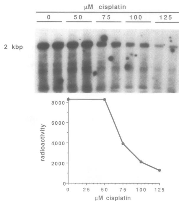
Figure 5. Quantitation of the PCR amplification of DNA purified from CHO cells incubated with cisplatin (fig. 4). \alpha\text{-}^{32}\text{P} -dCTP was included in the PCR step, and duplicate products were separated by electrophoresis and autoradiographed. The radioactivity was quantified and graphed.
