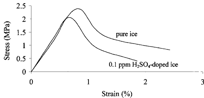
Fig. 1. Engineering stress–strain curves for undoped and \text{H}_2\text{SO}_4 -doped (0.1 ppm) ice single crystals with \theta = 80^{\circ} at -10^{\circ}\text{C} and an axial strain rate of 1 \times 10^{-6}\ \text{s}^{-1} .
