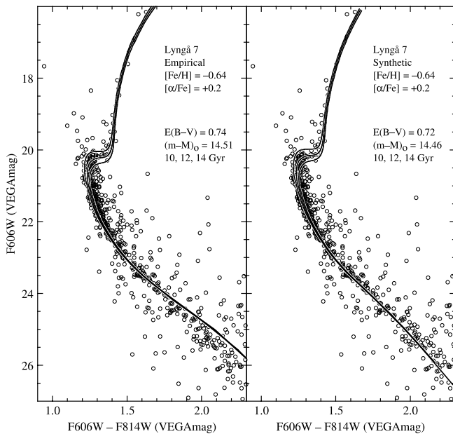
FIG. 26.—Same as Fig. 21, except that the CMD of Lyngå 7 is plotted for stars inside of 15'' from the cluster center.
