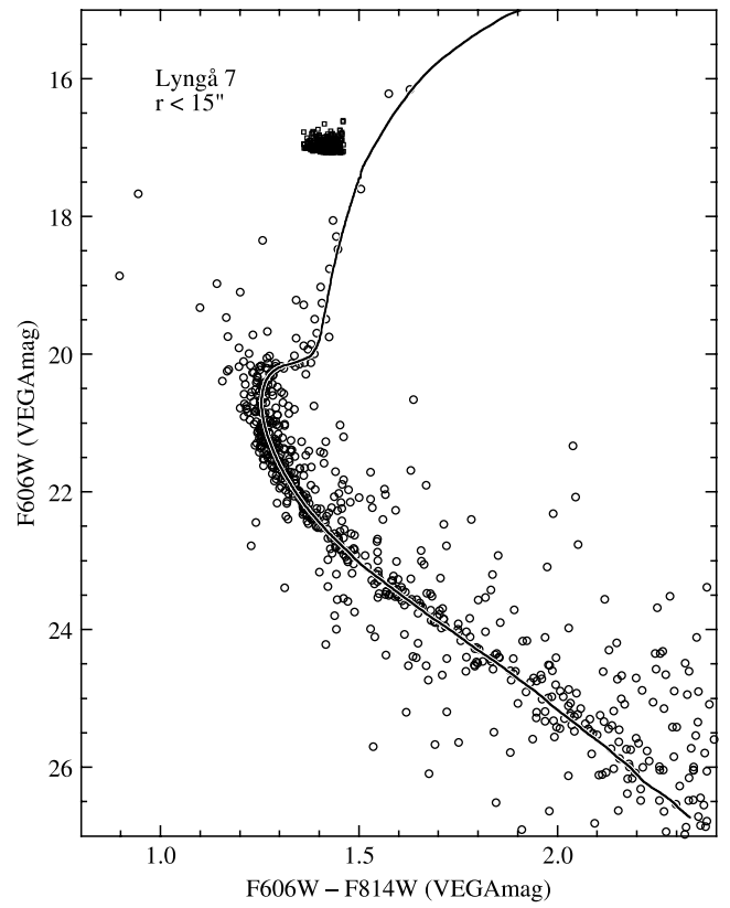
FIG. 15.—Same as Fig. 14, except that the CMD of Lyngå 7 is shown for stars less than 15'' from the cluster center.
