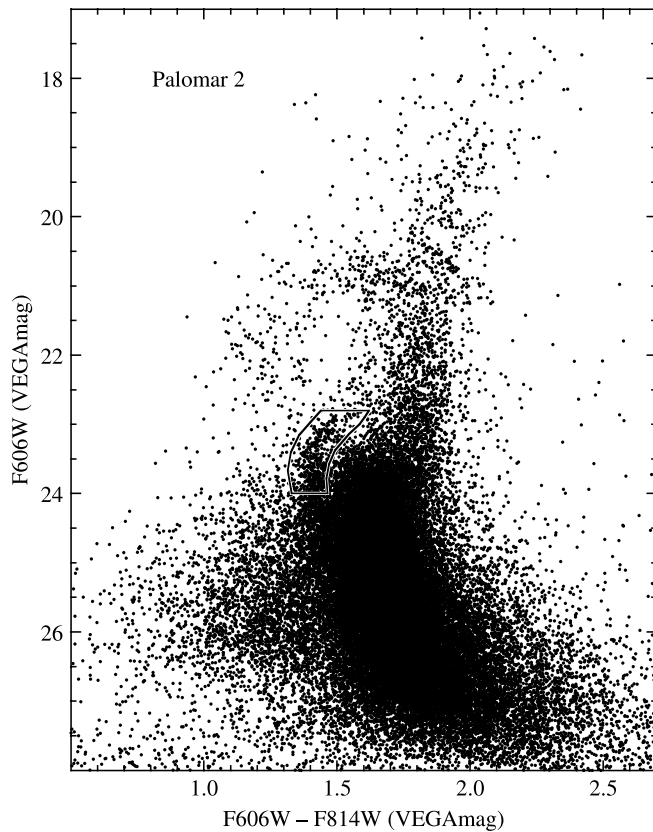
Fig. 18.— Left : CMD of Pal 2, with the main-sequence “extension” indicated by a boxlike region. Right : Location of stars (circles) in this box, relative to other stars in the cluster field. The circles are drawn at radii of 25'' , 50'' , 100'' , and 150'' and centered at (1800, 2400) pixels.
