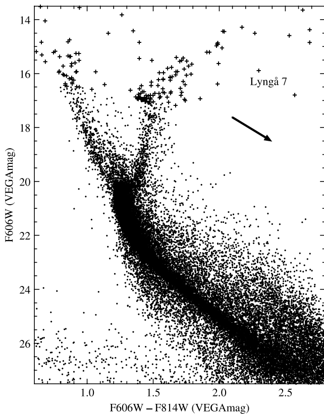
FIG. 7.—Same as Fig. 1, except that the CMD of Lyngå 7 is shown, containing 32,226 stars. The tidal radius for Lyngå 7 is not given in the Harris (1996) compilation. The arrow is the reddening vector for E(F606W - F814W) = 0.3 .
