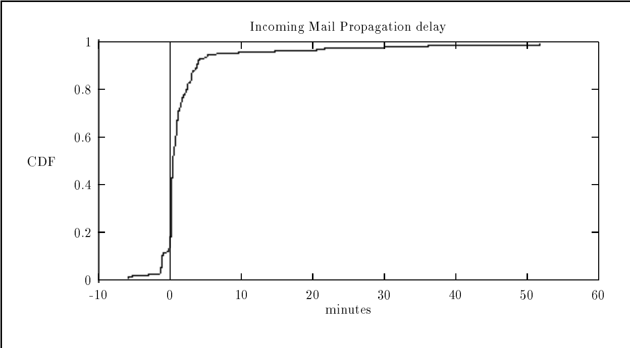
Figure 1: Time for a program or question submission to reach us. Over 90% of all mail reached us within five minutes. Two submissions took more than two hours (the sending machine crashed), and are not shown. Negative times are the result of clock differences.
