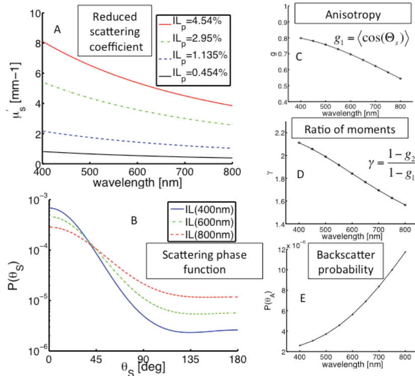
Fig. 2. Optical properties of Intralipid optical phantoms. A) shows reduced scattering coefficient vs. wavelength for selected IL dilutions. B) scattering phase function of PF: C) anisotropy, D) ratio of the first and second moments of the phase function, and the E) probability of large angle backscatter events. This study assumes that reduced scattering coefficient linearly relates to dilutions of IL, while PF-related parameters are dilution independent.
