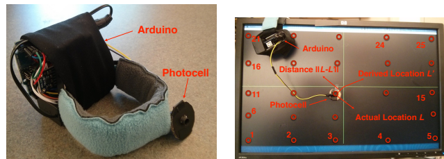
(a) Bracelet prototype (b) Localization setup
