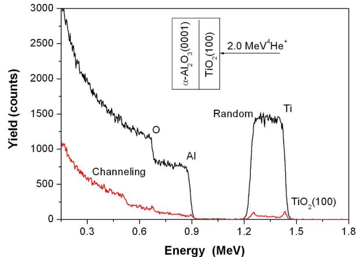
Figure 3. The 2 MeV 4 He + RBS/channeling spectra from a rutile-TiO 2 film with the thickness approximately 507 nm on the \alpha -Al 2 O 3 (0001) substrate. The aligned spectrum was taken with the beam directed along the (100) axis of the rutile-TiO 2 film. The film was deposited at 500°C under the O 2 gas pressure of 15 \times 10^{-3} Torr.
