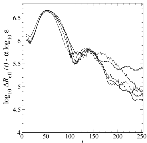
FIG. 7: Collapse of \Delta R_{\text{eff}} in Figure 6 using \Delta R_{\text{eff}}(\varepsilon, t) = \varepsilon^\alpha f(t) for \alpha \approx 2.05 . Note that the time domain is restricted to t \leq 250 , since \Delta R_{\text{eff}} \rightarrow 0 for t \gtrsim 250 (causing the log scale to be ill behaved).
