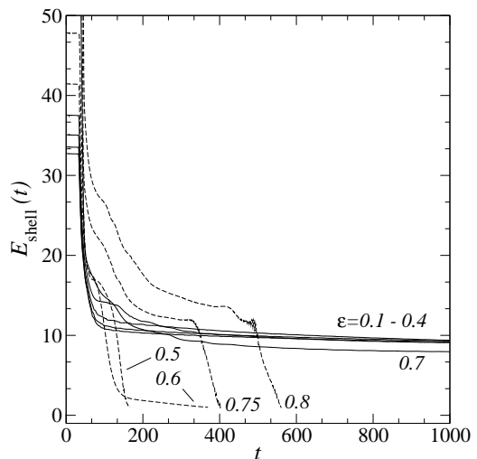
FIG. 5: Shell energy for bubbles of radius R_0 = 5.0 and steps \Delta\varepsilon = 0.05 (dashed lines for unstable cases).
