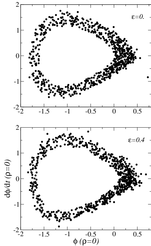
FIG. 8: Phase portrait between t = 0 and t = 1000 at \rho = 0 of a bubble entering an oscillon stage for R_0 = 2.0 and \varepsilon = 0 (top) and \varepsilon = 0.4 (bottom): the symmetric configuration to which asymmetric bubbles decay is an oscillon.
