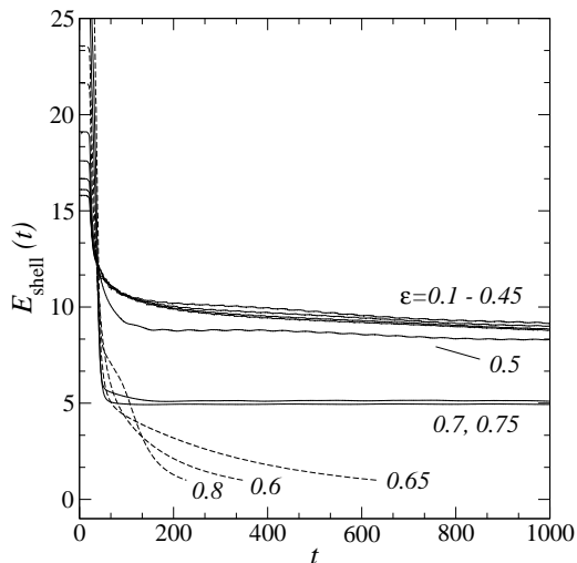
FIG. 3: Oscillon energy in a shell of radius R_s = 5R_0 , now for R_0 = 3.0 and 0.1 \leq \varepsilon \leq 0.8 , with steps \Delta\varepsilon = 0.05 . Dashed lines indicate unstable configurations.
