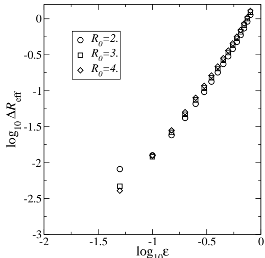
FIG. 1: Logarithm of the “effective radial dispersion” \Delta R_{\text{eff}}(t=0) vs. eccentricity \varepsilon for the ansatz (4). \Delta R_{\text{eff}} is clearly a good measure of asymmetry, increasing always monotonically with \varepsilon .
