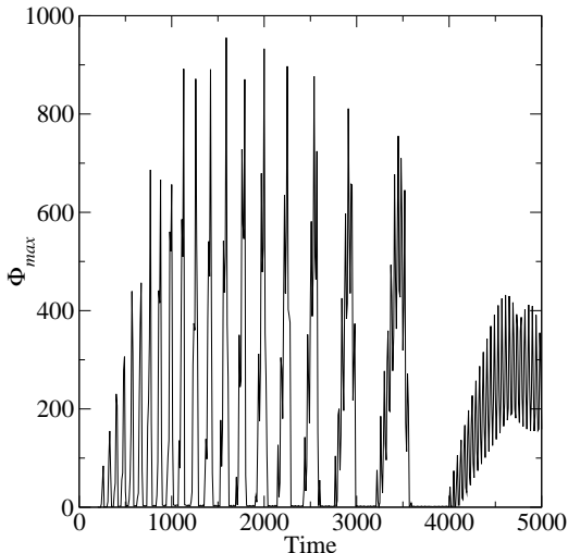
FIG. 10: A typical outcome of the linear stability analysis of the oscillon, showing here \Phi_{max} vs. time for \ell = 0 , n = 0 and m = 2 in Eq. (18). The radius of the initial bubble is R_0 = 2 .
