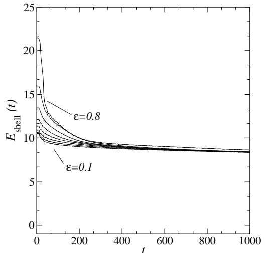
FIG. 2: Oscillon energy in a shell of radius R_s = 5R_0 for R_0 = 2.0 and 0.1 \leq \varepsilon \leq 0.8 , from bottom to top (only integer multiples of \varepsilon = 0.1 are shown).
