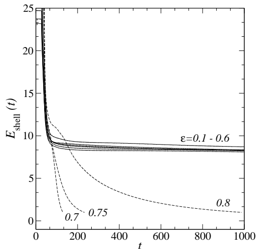
FIG. 4: Oscillon energy for R_0 = 4.0 and different \varepsilon , with steps \Delta\varepsilon = 0.05 (dashed lines are for unstable configurations).
