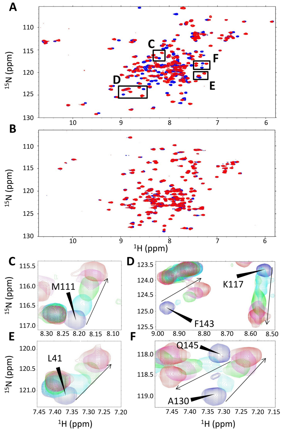
Fig 4. The DED1 R4 peptide interacts with calmodulin. (A) ^1\text{H} , ^{15}\text{N} -HSQC spectrum of calmodulin before (blue) and after addition of R4 (red), in the presence of \text{Ca}^{2+} . The peak shifts between the two spectra are indicative of a binding event. (B) Chelation of \text{Ca}^{2+} with EDTA abolishes the interaction. The spectra shown in blue and red are in the absence or presence of excess R4, respectively. The high degree of spectral overlap indicates there is no interaction between R4 and the protein. (C)-(F) Enlarged views of corresponding insets from panel A, showing examples of residues directly involved in binding to R4. Spectra depict the following R4:calmodulin ratios: blue—0:1; cyan—1:1; green—1.5:1; magenta 2:1; red—5:1. Other titration points were excluded for ease of visualization. Arrows indicate the direction in which the peaks shift.
