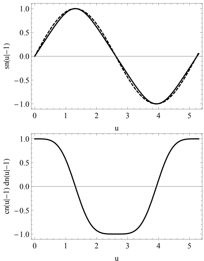
FIG. 10. Jacobi elliptic functions \text{sn}(u|-1) and its derivative \text{cn}(u|-1)\text{dn}(u|-1) are illustrated. The dashed line in the first panel corresponds to a regular sine function with a scaled argument: \sin(\frac{6}{5}u) .
