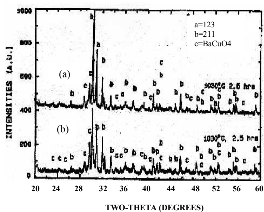
Figure 1. XRD pattern of (a) fine sample and (b) coarse sample quenched from 1030 ^{\circ}\text{C}
