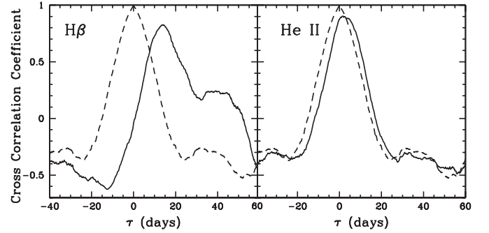
Figure 3. CCFs for the light curves. Dashed lines represent the autocorrelation function (ACF) of the continuum light curve, and solid lines show the CCFs for the emission lines.
