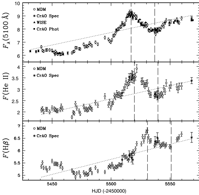
Figure 2. Complete light curves for Mrk 335 from our observing campaign. The top panel shows the 5100 Å flux in units of 10^{-15} erg s ^{-1} cm ^{-2} Å ^{-1} , the middle panel shows the flux in the He II \lambda 4686 region in units of 10^{-13} erg s ^{-1} cm ^{-2} , and the bottom panel shows the integrated H \beta \lambda 4861 flux, also in units of 10^{-13} erg s ^{-1} cm ^{-2} . Open circles denote observations from MDM Observatory and asterisks represent spectra taken at CrAO. Closed squares show the photometric observations from CrAO, and closed triangles represent photometric observations from WISE Observatory. Vertical dashed lines have been placed at two obvious features in the continuum to aid the eye. The vertical lines have been shifted by the measured He II and H \beta lag values (2.7 days and 13.9 days, respectively) to aid the eye in identifying the correct lag values for each emission line. Dotted lines show the trends that were subtracted before performing the cross-correlation analysis.
