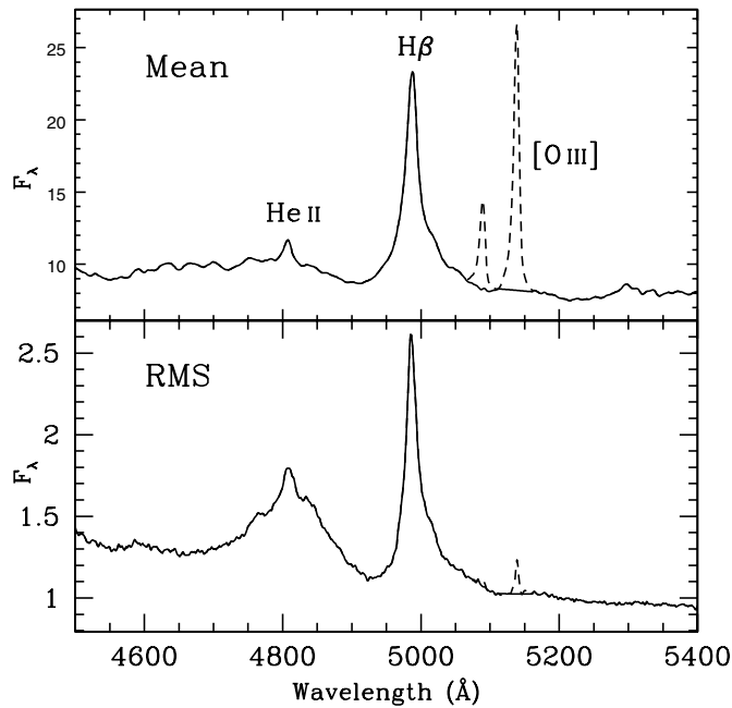
Figure 1. Flux-calibrated mean (top) and rms (bottom) spectra of Mrk 335 in the observed frame ( z = 0.02579 ). The flux density is in units of 10^{-15} \text{ erg s}^{-1} \text{ cm}^{-2} \text{ \AA}^{-1} . The dashed lines show the spectra before the [O III] narrow emission lines were removed; the solid line shows the spectra after the subtraction.
