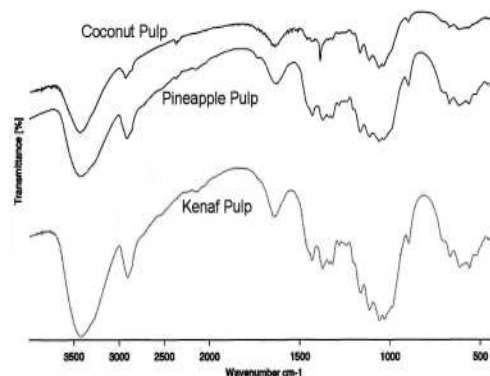
Figure 2. Infra red spectra of three pulp fibers.
