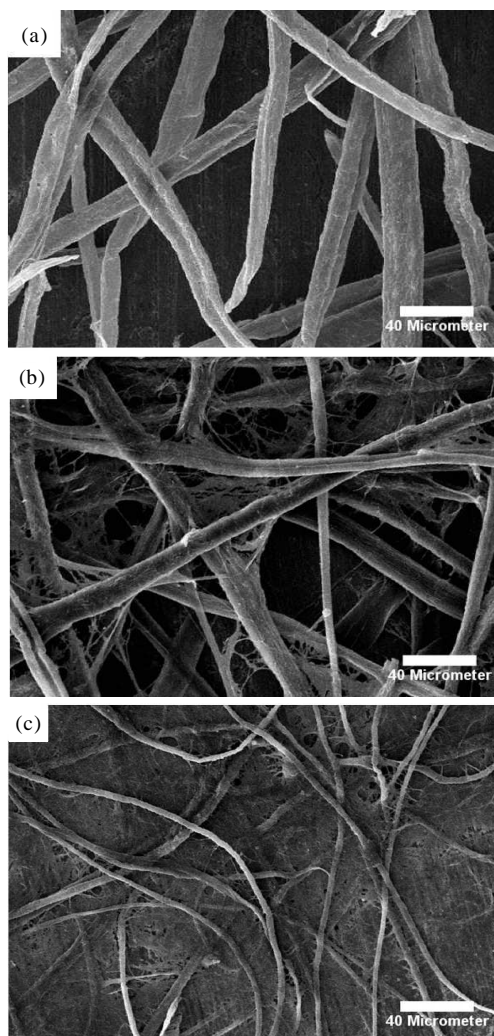
Figure 4. SEM image of three pulps fiber (a). Coconut (b). Kenaf and (c). Pineapple pulps
