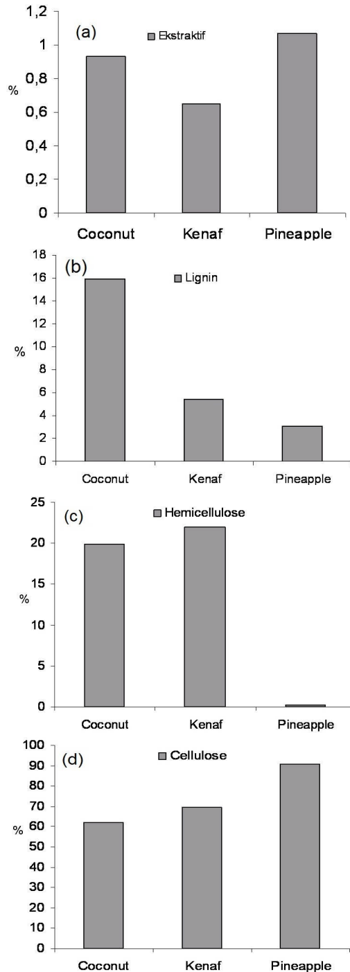
Figure 1. Chemical compositions (%) of three pulp fibers (a). Extractives, (b). Lignin, (c). Hemicellulose and (d). Cellulose
