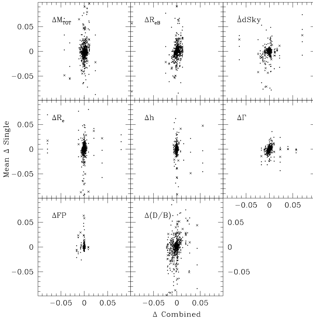
FIG. 12.—Profile combination algorithm and the precision of the derived parameters. The x-axis plots the residuals \Delta of the parameters derived using the fitting procedure with profile combination. \Delta d\text{Sky} and \Delta\Gamma are averaged over the four obtained values. The y-axis plots the mean of the residuals of the parameters derived by fitting each single independently as crosses, and the residuals of each fit as dots (see discussion in § 3.6).
