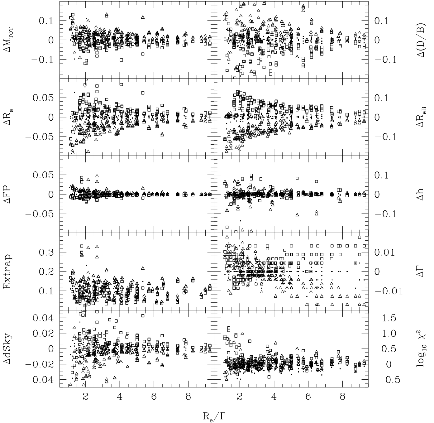
FIG. 11.—Effect of the choice of the PSF on the precision of the derived parameters. Open triangles for \gamma = 1.5 , dots for \gamma = 1.6 , and open squares for \gamma = 1.7 . Fits performed with the \gamma = 1.6 PSF overestimate (underestimate) magnitudes and half-luminosity radii of models constructed with \gamma = 1.5 ( \gamma = 1.7 ; see § 3.5). Note the expanded ordinate scale with respect to Figs. 4–9.
