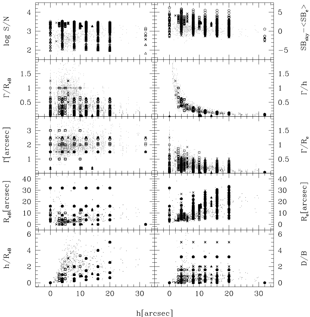
FIG. 1.—Parameter space of the R^{1/4} plus exponential profile of the Monte Carlo simulations discussed in Figs. 2–11. Crosses , models of Figs. 2–7 (see also Table 2). Filled triangles , models of Fig. 8. Open triangles , models of Fig. 9. Open squares , models of Figs. 10–11. Open pentagons , models of Fig. 12. Open hexagons , models of Fig. 13. The small dots show the position of the EFAR galaxies as determined in Paper III. The parameters of bulge-only models are shown with h = 0 . The parameters of disk-only models are shown at R_{eB} = 0 . See discussion in § 3.
