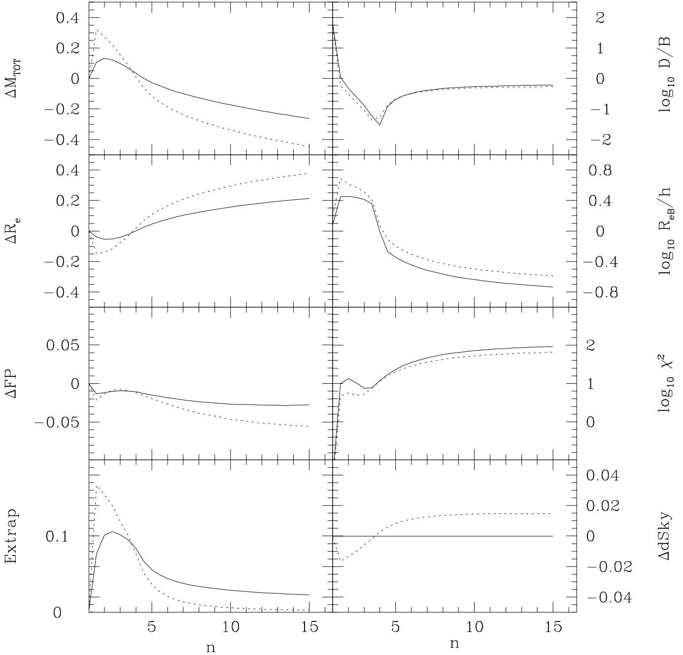
FIG. 15.—Relation between n and the parameters of the decomposition (see § 3.8). The solid curves refer to the results obtained with no sky-subtraction errors. The dotted curves show the results obtained when the sky-fitting algorithm is activated.
