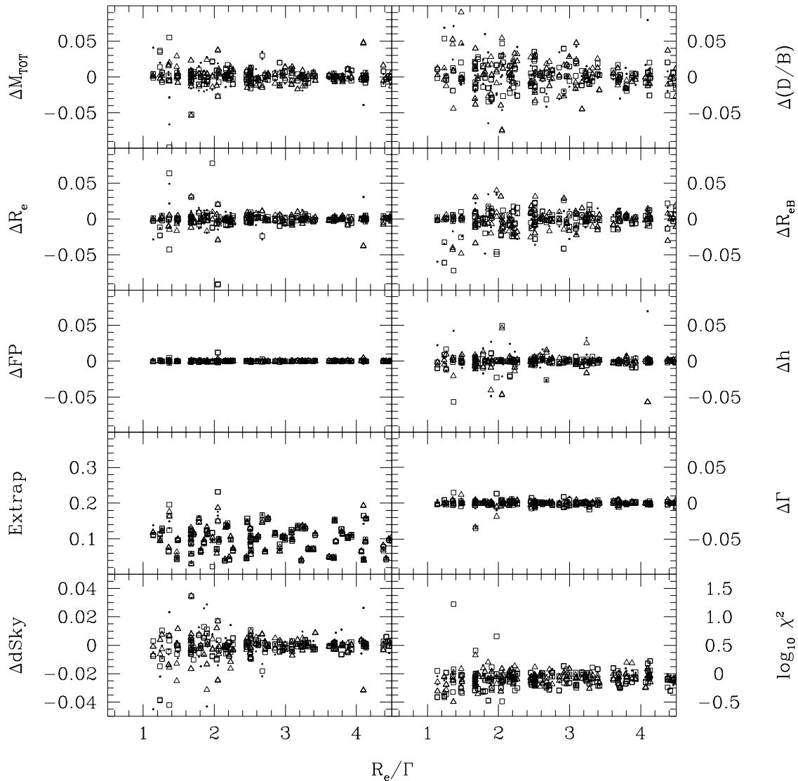
FIG. 10.—Effect of seeing and pixel sampling of the profiles on the precision of the derived parameters. Different symbols indicate different pixel sizes (small dot 0".4; triangles, 0".6; squares, 0".8). Note the expanded ordinate scale with respect to Figs. 4–9. See discussion in § 3.5.
