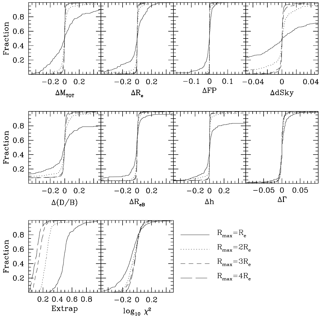
FIG. 8.—Effect of the radial extent of the profiles on the precision of the derived parameters. The cumulative distributions of the errors on the derived photometric parameters as derived from the simulations are shown for a range of R_{\max} values (solid lines, R_{\max} = R_e ; dotted lines, R_{\max} = 2R_e ; dashed lines, R_{\max} = 3R_e ; long-dashed lines, R_{\max} = 4R_e ). Good reconstructions are obtained when R_{\max}/R_e > 2 (see § 3.3).
