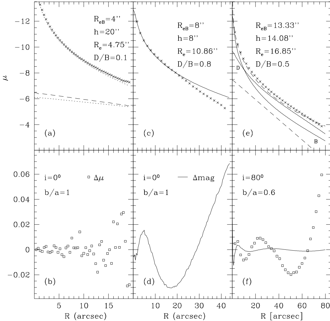
FIG. 3.—(a) Circular disk plus bulge model with D/B = 0.1 and h/R_{eB} = 5 (crosses). The dotted curves show the luminosity profiles \mu(R) = -2.5 \log I(R) of the bulge and the disk components, the dashed curve the fitted disk component. (b) Differences \Delta\mu (in mag arcsec -2 , open squares) between model surface brightness and the fitted one (dotted curve) (see § 3.1). (c) R^{1/4} fit (solid curve) to the surface brightness magnitude profile of a circular disk plus bulge model with D/B = 0.8 and h/R_{eB} = 1 (crosses, one point in every four). (d) Differences \Delta\text{mag} between the R^{1/4} integrated magnitudes and the fitted ones (solid curve; see § 3.1). Note that \Delta\text{mag} < 0.07 even if large deviations \Delta\mu are present. (e) Fit to the circularized profile of a flattened bulge plus an inclined disk model (see § 3.7). The luminosity profile of the model (crosses, one point in every four); the bulge and the disk components, with the listed parameters, are the solid curves) is best-fitted by an R^{1/4} plus exponential law (dashed curves) with parameters R_{eB}^f = 16''.34 , h^f = 13''.93 , (D/B)^f = 0.13 , R_e = 17''.51 . (f) Residuals \Delta\mu of the fit (open squares, one point in every four) and the differences between the growth curves \Delta\text{mag} (solid curve).
