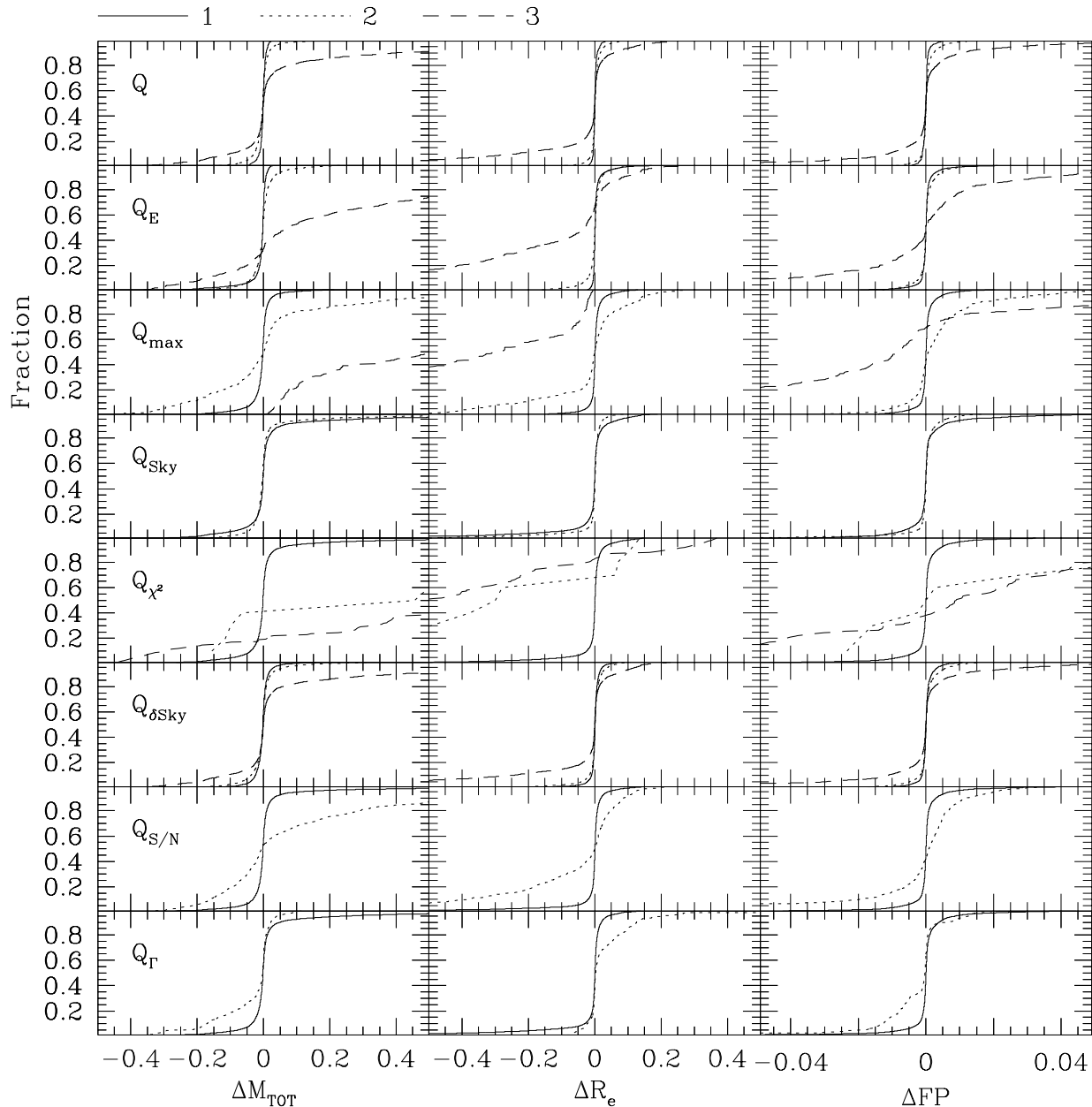
FIG. 16.—Precision of the reconstructed total magnitudes M_{\text{TOT}} , the half-luminosity radii R_e and the combined quantity FP = \log R_e - 0.3\langle SB_e \rangle . The cumulative distributions of the errors \Delta M_{\text{TOT}} , \Delta R_e , and \Delta FP derived from all the performed disk plus bulge fits with sky-correction algorithm activated are shown as a function of the different quality parameters defined in § 2.3. The solid lines plot the distributions when the parameters have value of 1, the dotted lines when the value is 2, the dashed lines when the value is 3. The distributions derived by selecting on the global quality parameter Q match the precision ranges identified in § 3.9.
