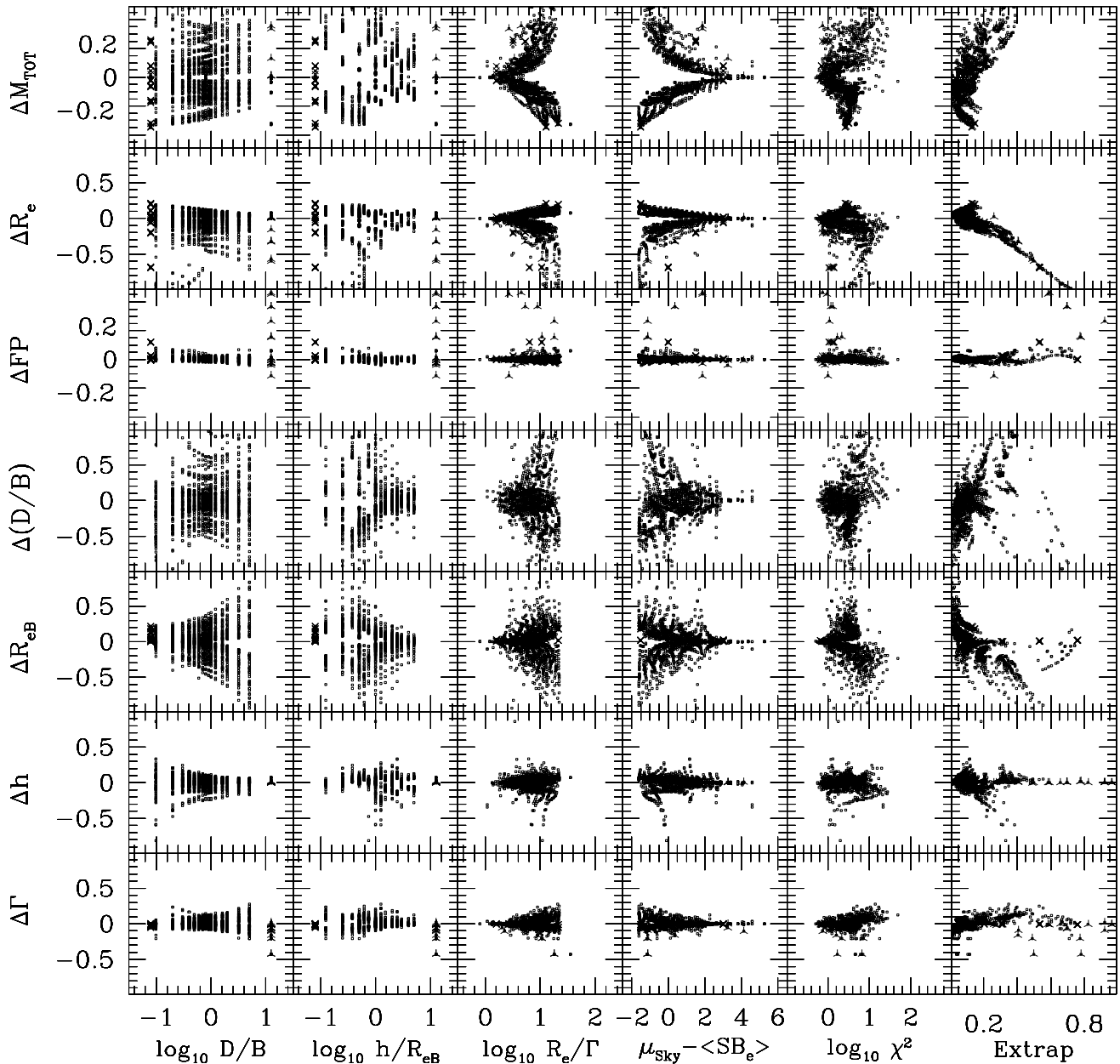
FIG. 6.—Biases introduced by a \pm 1\% sky-subtraction error. Quantities plotted as in Fig. 2. Models with D/B = 0 that have been fitted with two components are shown as crosses. Models with B/D = 0 that have been fitted with two components are shown as triangular crosses. Note the change of scale on the ordinate axis with respect to Fig. 2. See discussion in § 3.2.
