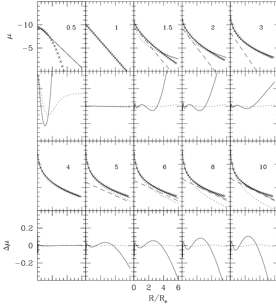
FIG. 14.—Fits to the R^{1/n} law. Two plots are drawn for each value of n (given in the top right corner). In the top plot the crosses (one point in every seven) show the luminosity profiles \mu(R) = -2.5 \log I(R) of the R^{1/n} law as a function of R/R_e . The dotted and dashed curves show the best-fitting R^{1/4} and exponential laws, respectively. In the bottom plot the residuals ( solid curves ) in mag arcsec ^{-2} from the fits to the R^{1/n} law are shown. The dashed curve shows the residuals (in mag) from the curves of growth (see discussion in § 3.8).
