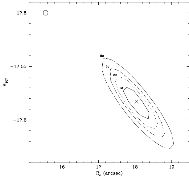
FIG. 5.—Illustration of the underestimation of the errors. The contours of constant \chi^2 near the minimum of an R^{1/4} fit to a h/R_{eB} = 0.5 , D/B = 0.1 disk plus bulge model. The cross shows the best-fit solution, the circle near the upper left corner gives the real parameters of the model. The errors estimated at the 5\sigma contour underestimate the differences between the model and the fit by a factor of 2 (see § 3.1).
