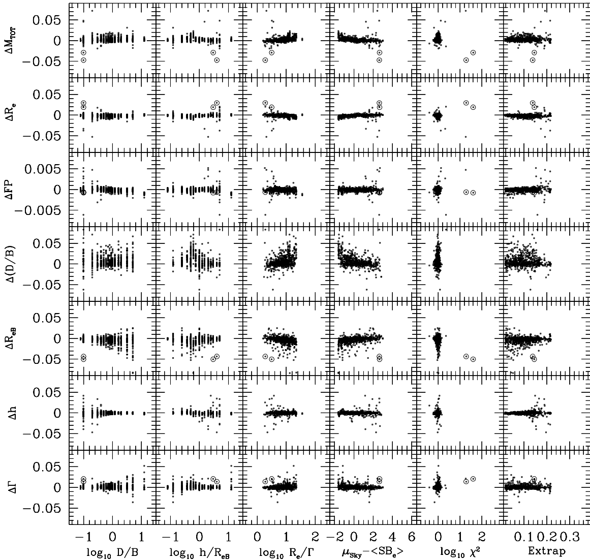
FIG. 2.—Reconstructed parameter space for the models indicated by the crosses in Fig. 1. No sky error is present. The quantities plotted on the y-axis are defined as \Delta M_{\text{TOT}} = M_{\text{TOT}} - M_{\text{TOT}}^f , \Delta R_e = \log R_e/R_e^f , \Delta FP = \Delta R_e - 0.3(\Delta M_{\text{TOT}} + 5\Delta R_e) = \Delta R_e - 0.3\Delta \langle SB_e \rangle , \Delta(D/B) = \log [(D/B)/(D/B)^f] , \Delta R_{eB} = \log R_{eB}/R_{eB}^f , \Delta h = \log h/h^f , \Delta \Gamma = \log \Gamma/\Gamma^f . On the x-axis, the first three boxes show the input parameters of the models in the logarithm units ( \log D/B , \log h/R_{eB} , \log R_e/\Gamma ). The last three boxes show the differences in magnitudes between the assumed sky value and the average effective surface brightness of the models ( \mu_{\text{sky}} - \langle SB_e \rangle ), the logarithm of the reduced \chi^2 , and the fraction of light extrapolated beyond R_{\text{max}} used in the determination of M_{\text{TOT}}^f . Models with D/B = 0 (pure R^{1/4} laws) are plotted at \log D/B = -1.1 and \log h/R_{eB} = -1.1 . Models with B/D = 0 (pure exponential laws) are plotted at \log D/B = 1.1 and \log h/R_{eB} = 1.1 . Models with D/B \neq 0 that have been fitted with one component are circled. See § 3.1 for a discussion of the results.
