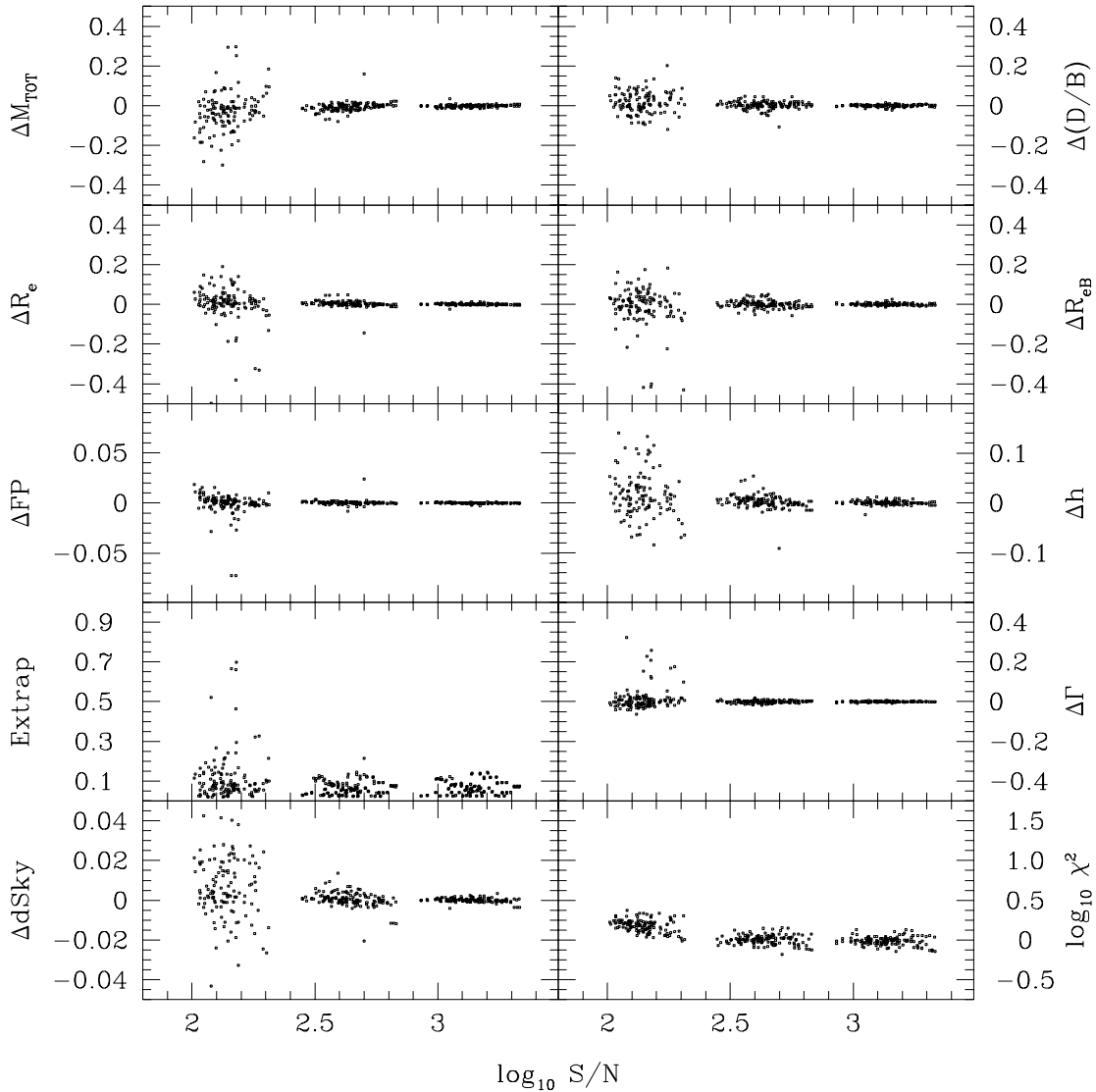
FIG. 9.—Effect of the signal-to-noise ratio of the profiles on the precision of the derived parameters. Good reconstructions are obtained when S/N > 300 (see § 3.4). Note the change of scale on the ordinate axis with respect to Fig. 2.
