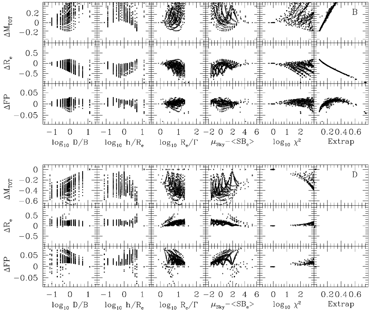
FIG. 4.—Effects of fitting disk plus bulge test profiles by either a single bulge ( first three rows of plots ) or a single disk ( last three rows of plots ) model. The test models are indicated by the crosses of Fig. 1. \Delta M_{\text{TOT}} , \Delta R_e , and \Delta FP are defined as in Fig. 2, x-axis as in Fig. 2. See § 3.1 for the a discussion of the results. Note the change of scale on the ordinate axis with respect to Fig. 2.
