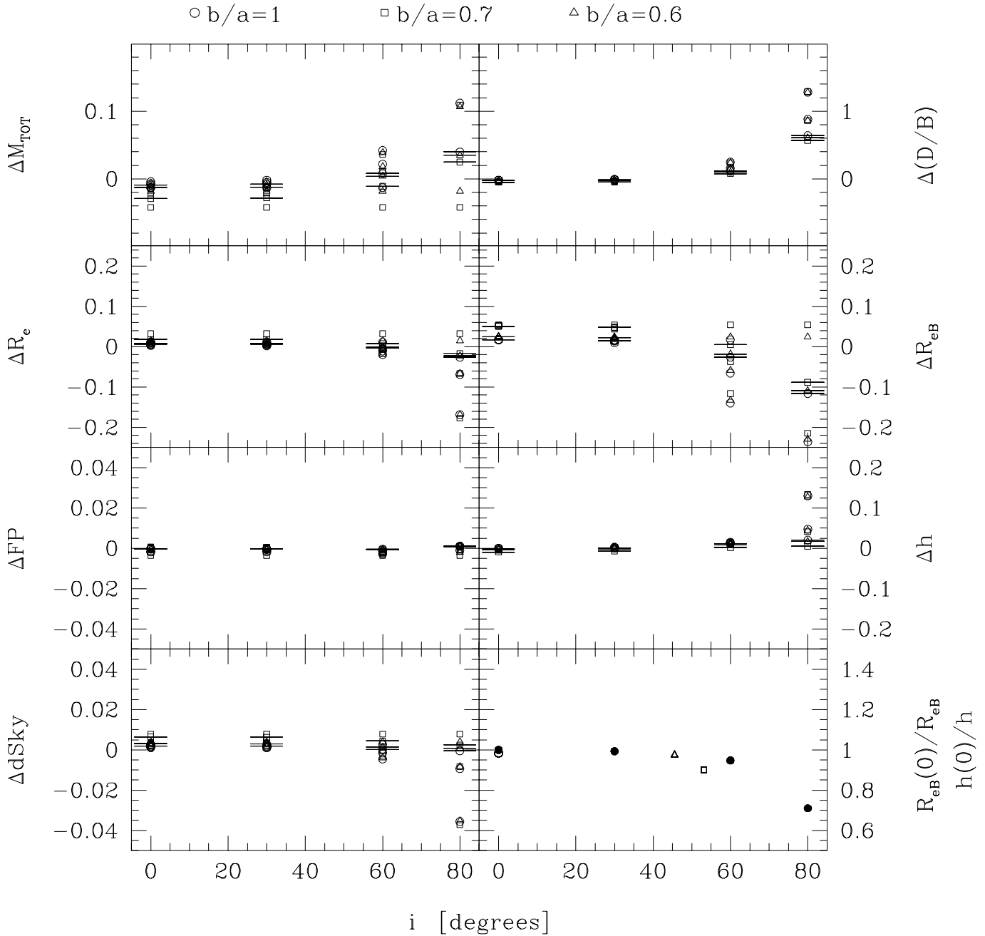
FIG. 13.—Reconstructed parameters of the bulge plus disk models as a function of the inclination i of the disk. Different symbols indicate different flattenings of the bulge. The horizontal bars show models with D/B = 0.5 . The plot at the bottom right shows the scale lengths of the flattened bulge ( open symbols ) or of the inclined disk ( filled symbols ) as a function of the flattening angle [ i = \arccos(b/a) ] or of the inclination angle, normalized to the b/a = 1 or i = 0^\circ values. Good reconstructions of the parameters are obtained when the inclination is less than 60^\circ (see § 3.7).
