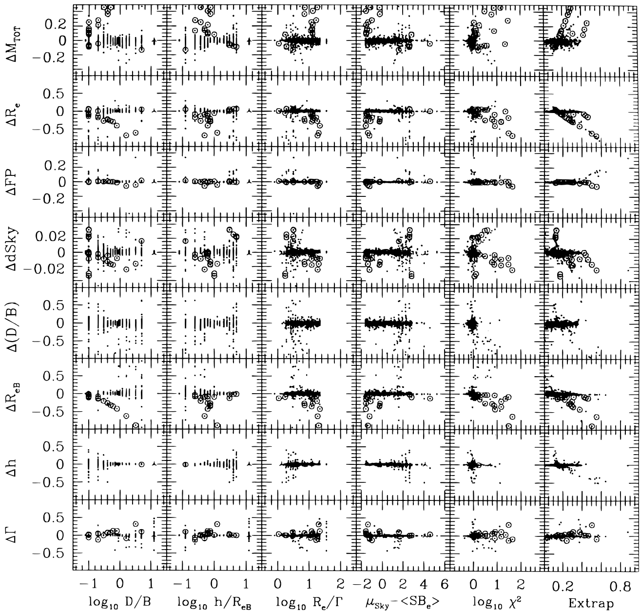
FIG. 7.—Effects of the sky-fitting algorithm. The parameters of the models of Fig. 6 with the sky-subtraction errors of 0, \pm 1\% , \pm 3\% , are reconstructed using the sky-fitting algorithm. Quantities and symbols plotted as in Figs. 2 and 6. In addition, the difference \Delta d\text{Sky} = d\text{Sky}/\text{Sky} - d\text{Sky}^j/\text{Sky} on the sky correction is plotted. Note the change of scale on the ordinate axis with respect to Fig. 2. See discussion in § 3.2.
