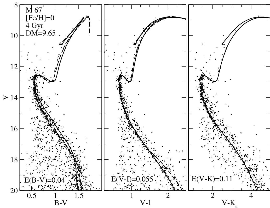
FIG. 9.—CMDs of M67 in B - V and V - I (Montgomery et al. 1993) and V - K_s (GS03). Isochrones with [\text{Fe}/\text{H}] = 0 at 4 Gyr are shown using synthetic ( solid line ) and VC03 ( dashed line ) colors. A He-burning track with M = 1.25 M_{\odot} at [\text{Fe}/\text{H}] = 0 is plotted to indicate the predicted level of the red clump.
