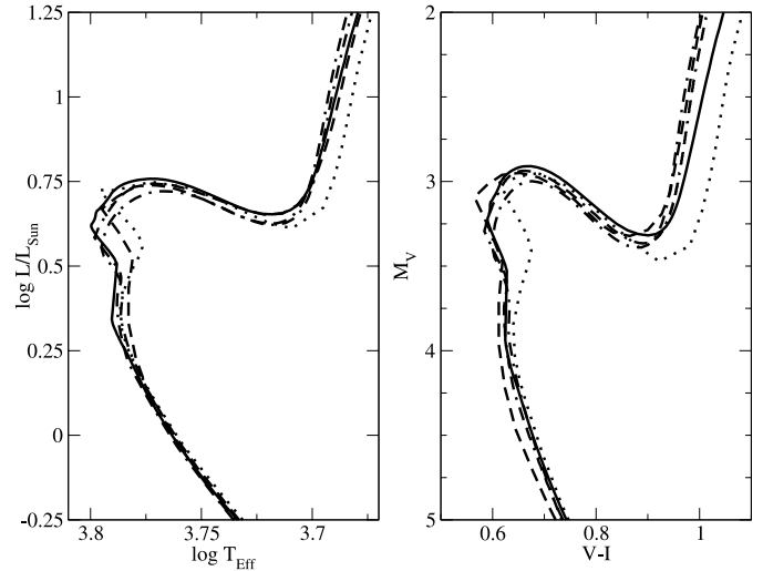
FIG. 5.—Same as Fig. 4, but focused on the region near the main-sequence turn-off. [See the electronic edition of the Supplement for a color version of this figure.]
