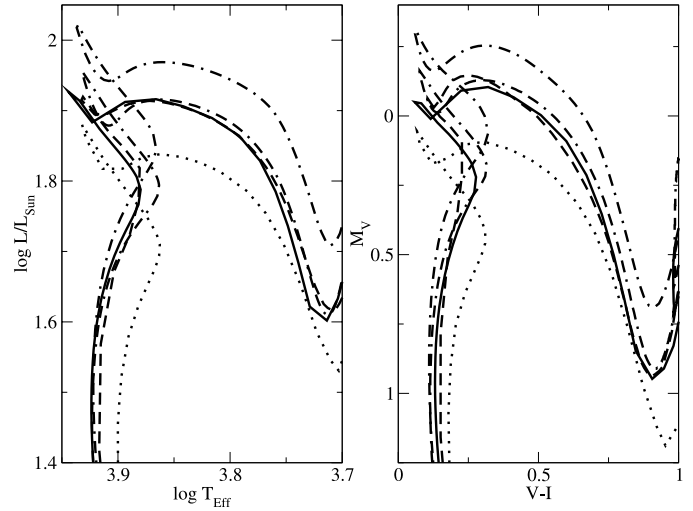
FIG. 3.— Same as Fig. 2, but focused on the region near the main-sequence turnoff. [See the electronic edition of the Supplement for a color version of this figure.]
