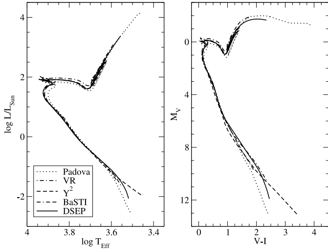
FIG. 2.— Isochrones at [\text{Fe}/\text{H}] \sim +0.15 and an age of \sim 625 Myr. The Padova, BaSTI, and DSEP isochrones show the He-burning phase but the others do not. Good agreement exists among all the isochrones except for Padova, which is cooler and fainter around the main-sequence turnoff. [See the electronic edition of the Supplement for a color version of this figure.]
