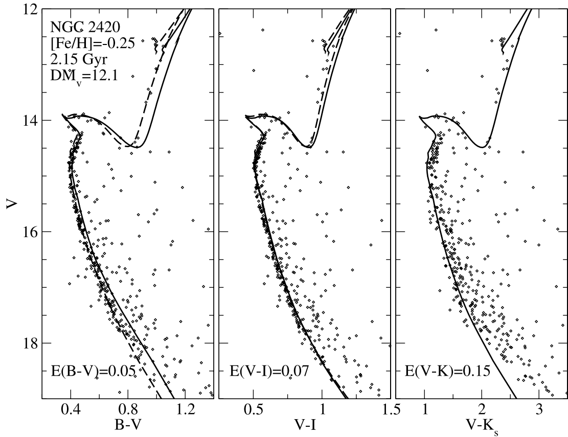
FIG. 8.—NGC 2420 from GS03 along with an isochrone interpolated to [\text{Fe}/\text{H}] = -0.25 and 2.15 Gyr. The isochrone is shown with synthetic colors ( solid line ) and VC03 colors ( dashed line ). Also shown is a 1.5 M_{\odot} He-burning track interpolated to [\text{Fe}/\text{H}] = -0.25 .
