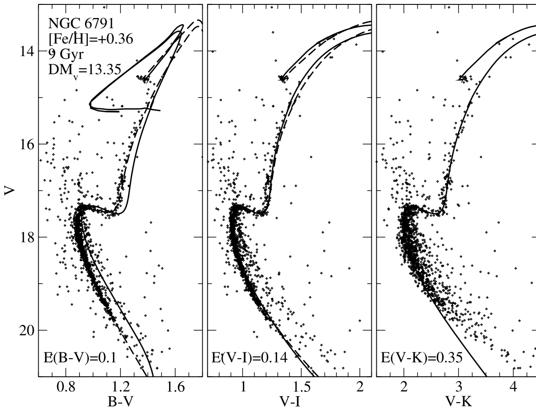
FIG. 10.— B - V , V - I , and V - K CMDs of NGC 6791 from Stetson et al. (2003) and Carney et al. (2005). Plotted on top of the data are isochrones with [\text{Fe}/\text{H}] = +0.36 at 9 Gyr in synthetic (solid line) and VC03 (dashed line) colors. A 1 M_{\odot} He-burning track of the same composition is plotted to indicate the predicted location of the red clump.
