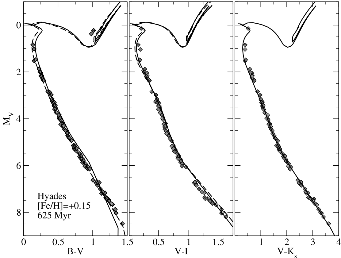
FIG. 7.—Hyades in B - V and V - I from de Bruijne et al. (2001) along with V - K_s from Pinsonneault et al. (2004). Along with the data, an isochrone with [\text{Fe}/\text{H}] = +0.15 at 625 Myr is plotted using the synthetic colors (solid line) and VC03 colors (dashed line).
