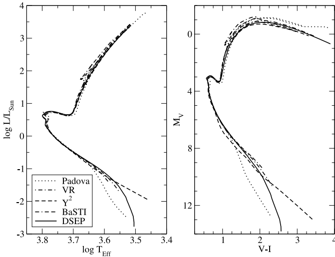
FIG. 4.—Solar metallicity isochrones at 4 Gyr. The Padova and BaSTI isochrones include the He-burning phase but the others do not. There is remarkable agreement in the H-R diagram between the tip of the red giant branch and \log L/L_{\odot} = -1 . Below this point, the range of masses plotted and the adopted EOS cause large differences. There is good agreement in the color-magnitude diagram between M_V = 6 and 0 but beyond this the mass range plotted, the underlying physics, and the choice of color transformation cause significant discrepancies. [See the electronic edition of the Supplement for a color version of this figure.]
