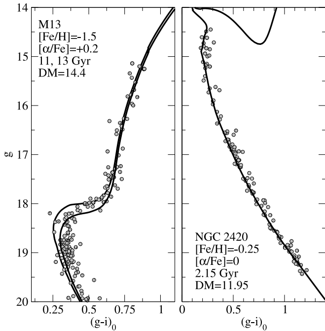
FIG. 11.—Dereddened g-i CMDs of M13 and NGC 2420 from Lee et al. (2007) plotted along with isochrones of appropriate age and metallicity transformed to the SDSS ugriz system.
