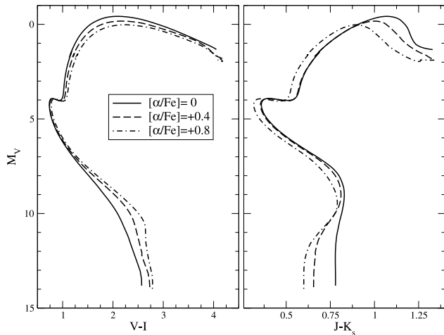
FIG. 1.— Influence of \alpha -enhancement on broadband V - I and J - K_s colors at [\text{Fe}/\text{H}] = 0 . The underlying isochrones shown are all scaled-solar composition with [\text{Fe}/\text{H}] = 0 at 10 Gyr. Only the color transformations include \alpha -enhancement. See the text for a discussion of the trends shown in the figure.
