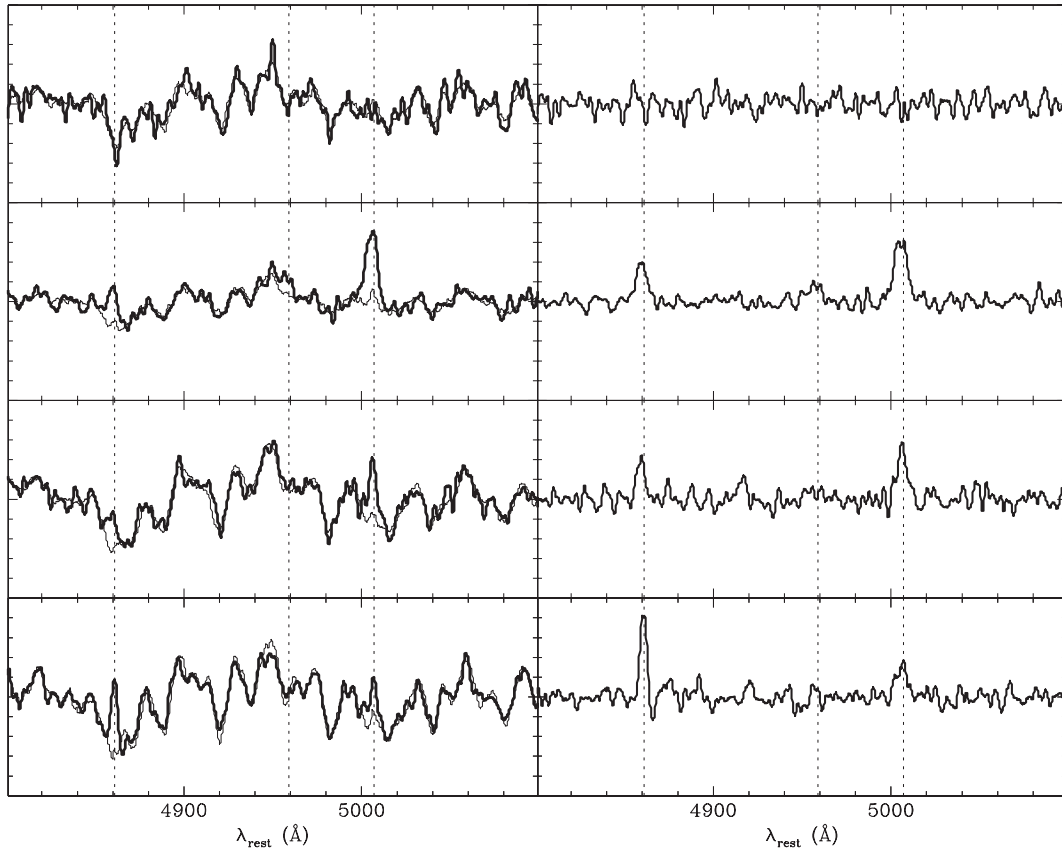
FIG. 4.—Some illustrative examples of the emission-line measurements. In the left-hand panels are shown the observed spectrum ( thick line ) and the best-fit Vazdekis (1999) model ( thin line ). The ratio spectrum, from which the line measurements are derived, is shown in the corresponding right-hand panel. Vertical dotted lines indicate the expected location of the H \beta and [O III] lines. At the top, a spectrum with no measurable emission is shown; in the lower three panels, spectra with weak to moderate emission. Note the substantial range of H \beta -to-[O III] ratios among these examples.
