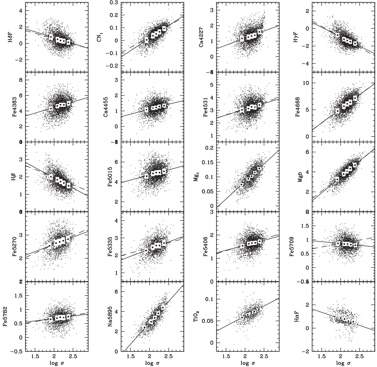
FIG. 8.—Our line-strength– \sigma relations for each index. The line strength and velocity dispersion for the galaxies ( points ) are sorted into five bins by increasing velocity dispersion ( black boxes outlined in white ). Solid lines are the slopes from the linear regression of line strength on \log \sigma . Dashed lines represent slopes predicted from our derived trends of [\alpha/\text{Fe}] , [\text{Z}/\text{H}] , and age with velocity dispersion in § 6 (see text in that section).
