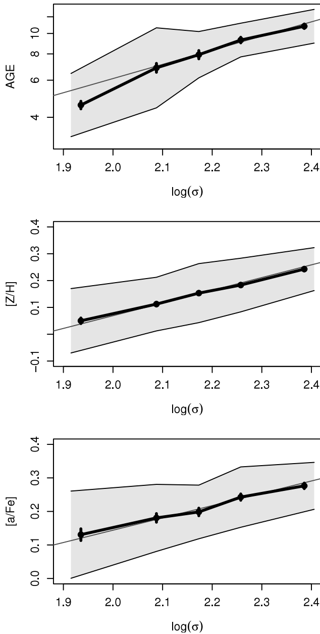
FIG. 13.—Fundamental scaling relations of the population parameters with \sigma . The thick line shows average age, metallicity, and [\alpha/Fe] determined in bins of velocity dispersion, using the grid inversion method. The set of line indices employed is the same as that in the slopes method. For comparison, the linear relations obtained from the slopes method are overplotted as the thin line, with zero point adjusted to match the grid inversion results. The shaded regions indicate the maximum internal scatter estimated in § 6.5.
