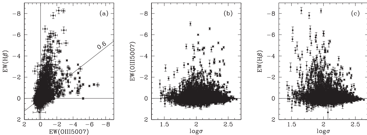
FIG. 5.—Emission measurements at [O III] \lambda 5007 and H \beta as a function of velocity dispersion, \sigma .
