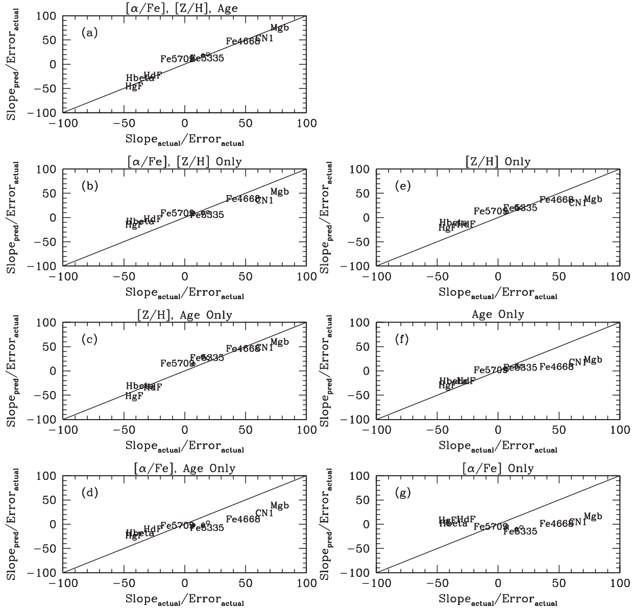
FIG. 10.—Comparison of the predicted index- \sigma slopes ( vertical axis ) with the observed slopes ( horizontal axis ) for different combinations of the three stellar population parameters. Labels indicate the results for each of the 12 line-strength indices. The diagonal line indicates perfect agreement between model-predicted and measured slopes. Note that both model-predicted slopes and measured slopes are normalized by the formal error in the measured slope. Thus, the vertical offset from the line indicates the degree to which the model fails to predict the observed slope. Panel (a) shows our default solution in which [\alpha/\text{Fe}] , [\text{Z}/\text{H}] , and \log(\text{age}) are scaled with \log \sigma . The model predictions for Fe5709 deviate from the observed slope at a high significance level (compare with Fig. 8). Note, however, that Fe5709 is discrepant in all panels. Panels (b)–(d) show the comparisons when we assume no trend with \sigma for age, [\alpha/\text{Fe}] , and [\text{Z}/\text{H}] , respectively. In these cases, there are multiple indices that deviate strongly from the model predictions. For example, if we assume no age gradient (panel [b]), we cannot simultaneously reproduce the slopes of Mg b and CN 1 and the Balmer lines. The fits are considerably poorer when only one parameter is allowed to vary, as in panels (e)–(g).
