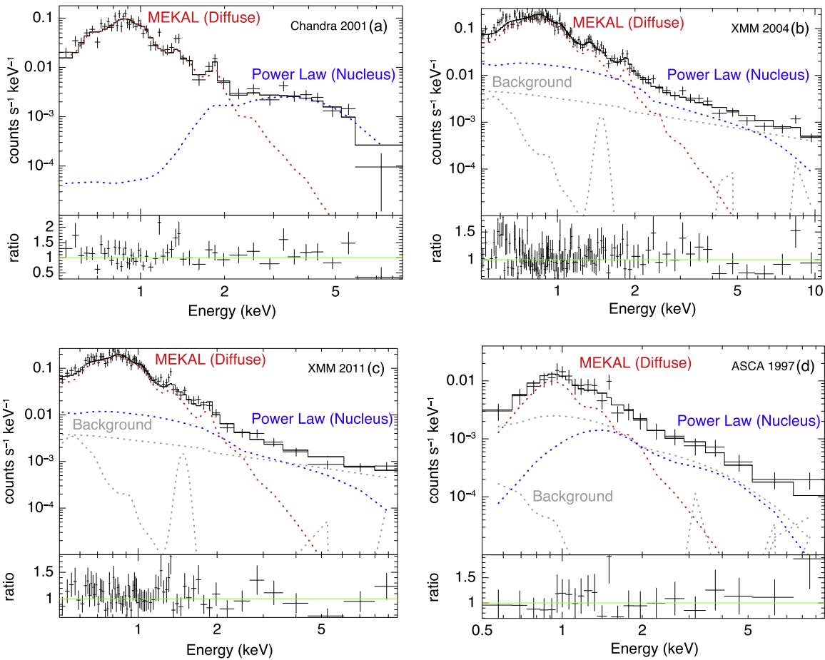
Figure 2. X-ray spectra including model fits and residuals, for four X-ray observations of He 2–10. Each component of the model fitted to the data are shown as dotted lines: the diffuse VMEKAL component (red) and nuclear power law (blue). For the Chandra observation (a) the background was subtracted before spectral fitting, while for the XMM (b), (c) and ASCA (d) observations, the background spectra are fitted by a model (shown by the gray lines) simultaneously with fitting of the observed source spectrum. There is a strong and significant detection of the hard nuclear power-law component in the 2001 Chandra (a) observation (clearly visible as a point source in Figure 1). The hard component is significantly weaker in the XMM observations (b), (c) indicating variability by approximately an order of magnitude. The hard component is also detected, at lower significance, in the 1997 ASCA spectrum (d).
