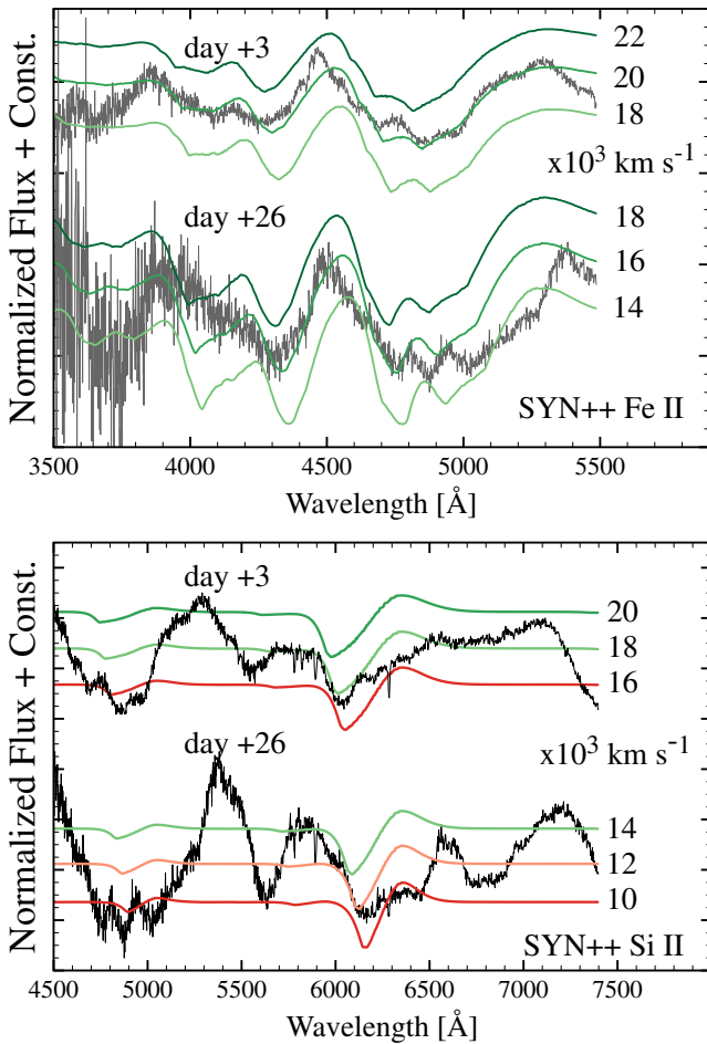
Figure 10. Individual ion fits for Fe II and Si II. For both the day +3 and day +26 spectrum, Fe II is most consistent with projected Doppler velocities of 20,000 km s -1 and 16,000 km s -1 , respectively. The projected Doppler velocities for Si II at these same epochs is ~2000–4000 km s -1 below those of Fe II.
