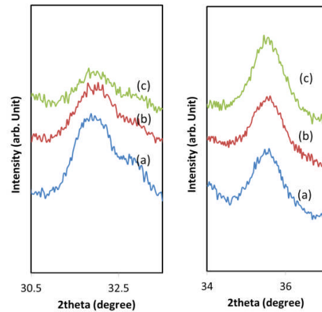
Figure 2. Detail diffraction pattern of HAP ( 30.5^\circ - 33.5^\circ ) and Fe_3O_4/\gamma-Fe_2O_3 ( 34^\circ - 37^\circ ) principal peaks for (a). K30; (b). K40 and (c). K50 samples.
