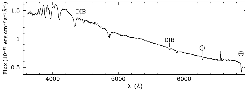
Figure 2. Flux-calibrated spectrum of LS IV–08°3, obtained UT 2002 April 3 at the Steward Observatory 2.3 m telescope, including higher-order Balmer lines. Absorption bandheads at \lambda 6277 and \lambda 6867 are telluric; absorption features at \lambda 4430 (near the stronger He I \lambda 4471 feature) and \lambda 5780 are diffuse interstellar bands.
