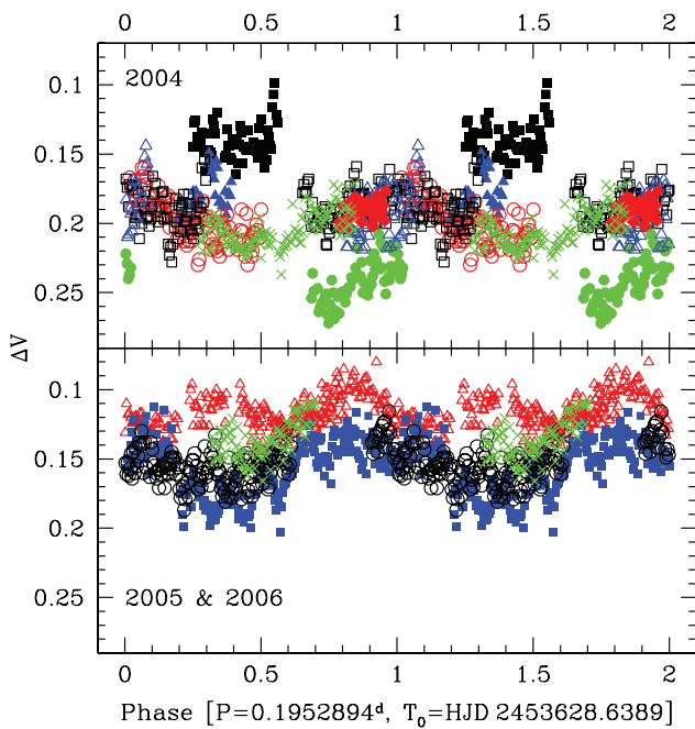
Figure 6. Folded differential light curve of LS IV–08°3, based on the RV ephemeris. The typical error of a single observation is \pm 0.02 mag. Different symbols indicate different observing nights. Data are plotted twice for phase continuity. Top: observations from 2004—July 26 filled diamond (colored red in online journal); August 1 cross (green); August 7 filled square (black); August 9 filled triangle (blue); August 16 open circle (red); August 22 open square (black); August 31 filled circle (green); September 18 open triangle (blue). Bottom: observations from 2005—July 15 cross (green); July 20 open circle (black); July 23 filled square (blue)—and 2006—May 27 open triangle (red). (A color version of this figure is available in the online journal)
