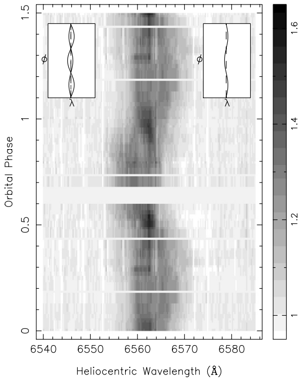
Figure 5. A trailed-spectrogram representation of the variations in the H\alpha emission profile from the HET-HRS. Wavelengths are heliocentric. Orbital phase increases upwards, with 1.5 cycles being shown for continuity (data are repeated). Intensities are in units of the continuum level and are indicated by the calibration strip along the right side of the main panel. The first inset (upper left) is intended as a guide to identifying the two distinct emission components moving in antiphase. The second inset (upper right) shows the single RV curve, with reduced amplitude, resulting from the analysis of the low-resolution MDM data. See the text for details and cautions.
