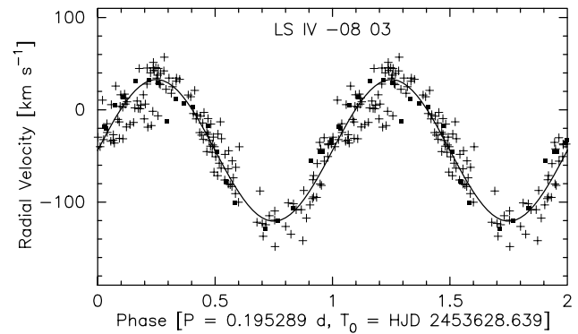
Figure 3. H \alpha radial velocities used in the analysis, folded on the best-fitting period, with the sinusoidal fit superposed. Crosses: MDM velocities; filled squares: HET-HRS velocities. Two cycles are shown for continuity.
