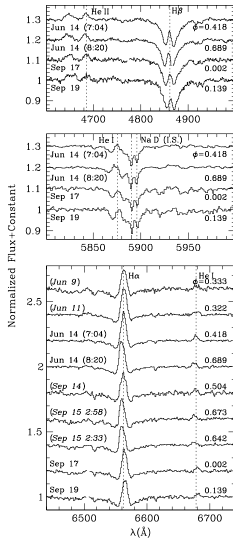
Figure 1. KPNO 2.1 m Goldcam spectra of LS IV−08°3 showing the variable nature of the emission components at Hβ (top), He I 5875 Å partly blended with interstellar Na I D lines (middle), and Hα/He I 6678 Å (bottom). Dates and times are UT 2003; times correspond to mid-exposure and are heliocentric. Phases corresponding to the ephemeris in Section 2.1.4 are also indicated. Dates that are italicized in parentheses in the bottom panel do not have corresponding data for Hβ and He I 5875 Å. Dotted lines show the laboratory wavelengths of the labeled transitions; the spectra themselves are plotted using observed (topocentric) wavelengths. Several gaps in the spectra result from cosmic ray removal.
