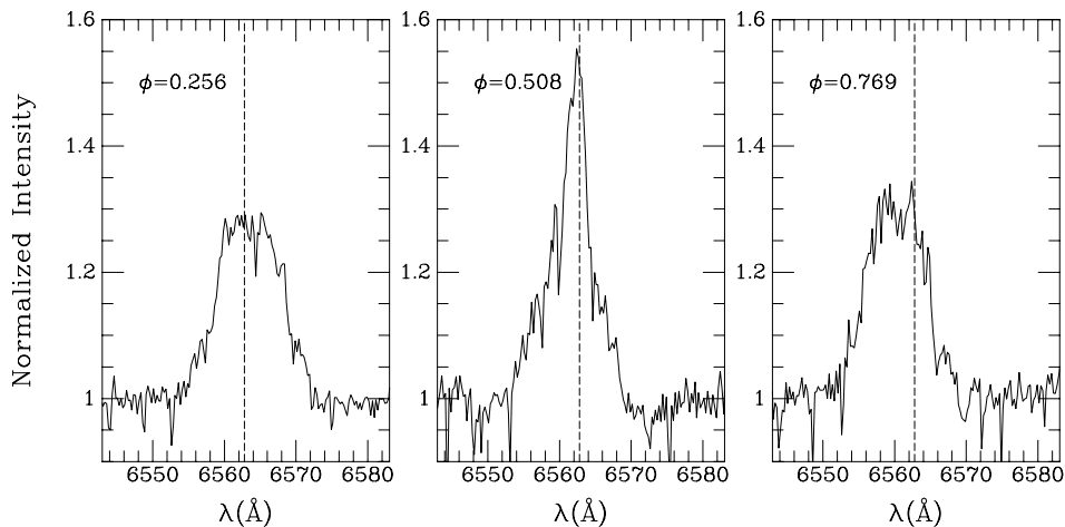
Figure 4. HET-HRS spectra showing only the emission component of the H\alpha line, for selected orbital phases: left: \phi = 0.256 (2004 May 24); middle: \phi = 0.508 (2007 April 19); right: \phi = 0.769 (2004 May 29). Wavelengths are heliocentric. The spectra have been “stretched” to make the emission EW uniformly 3.0 \text{ \AA} (see Section 2.2). The variation of the emission profile is evident. The dashed vertical line in each panel indicates the laboratory wavelength of H\alpha . The narrow absorption lines, which are stationary in the topocentric frame, are telluric.
