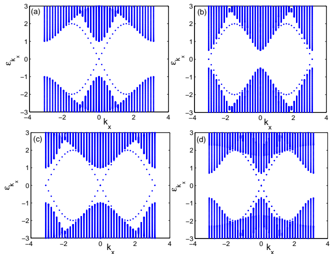
FIG. 2: (Color online) Excitation spectrum of Hamiltonian H on a cylinder for \mu = 0, t = 1, \lambda = 1 . Panel (a), C_+ = 1 : \Delta = 2, u_{cd} = 3 ; Panel (b), C_+ = -1 : \Delta = 2.5, u_{cd} = 2 ; Panel (c), C_+ = 0 : \Delta = 2, u_{cd} = 1 ; Panel (d), C_+ = 2 : \Delta = 0.8, u_{cd} = 1.5 . Note that the bulk gap scales as \min(\lambda, \Delta) . The number of lattice sites (N_x, N_y) = (40, 100) .
