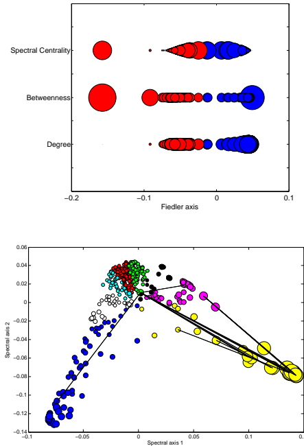
FIG. 3: 1-spectral centralities in example dense weighted networks. Top: A comparison of degree, betweenness and spectral centralities of the roll call network of the 111 th U.S. House of representatives. Color denotes party affiliation (red=Republican, blue=Democrat) while size is proportional to the relevant statistic. Nodes are ordered by the Fiedler vector. Bottom: The S&P 500 network given by its two dimensional spectral embedding where node size is proportional to spectral centrality. Coloring is given by an 8-cluster spectral clustering using two eigenvectors, the edges are the 30 edges with the highest spectral centrality.
