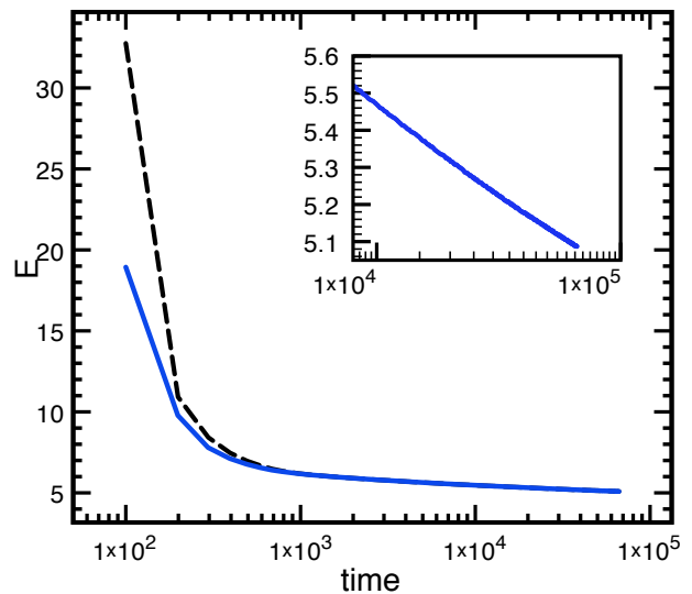
FIG. 6: (Color online) Time evolution of the total energy (dashed) and of the energy within a sphere of R = 4 for a \beta = 0.01 oscillon. After a quick shedding of a large amount of energy, the onset of the oscillon stage at time t \sim 10^3 is characterized by a very slow energy decay accurately fitted by \dot{E}(t) = -c_1 t^{-c_2} , where c_2 \simeq 1.2 . The inset shows the numerical value of the energy and the fitted curve (indistinguishable) for t \geq 10^4 .
