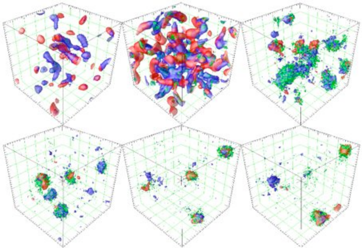
FIG. 19: (Color online) Local observables for a SU(2) quench at g = 4.0 on a lattice of volume 28.8^3 m_s^{-3} . Time slice isosurfaces corresponding to the times labeled in figure 18. Isosurfaces are twice their global averaged values, except for \Phi^\dagger\Phi = 0.5 . These particular configurations are large amplitude and decay quickly due to interactions with the propagating modes surrounding them. The full simulation can be viewed here .
