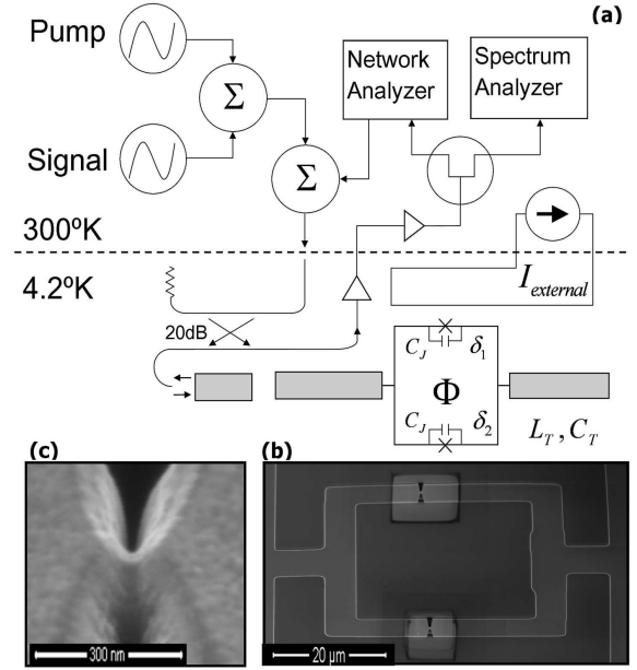
FIG. 1: (a) The device and the experimental setup. The SSR is made of two identical stripline sections of length l_T/2 = 110\text{mm} , each having inductance L_T and capacitance C_T per unit length and characteristic impedance Z_T = \sqrt{L_T/C_T} = 50\Omega . The stripline sections are connected by a SQUID consisting of nanobridge type weak links. All measurements are done at liquid Helium temperature 4.2 K, where the device is placed inside a copper package, which is internally coated with Nb (to reduce surface resistance and to provide magnetic shielding). (b) SEM micrograph of the SQUID (tilted view). The loop area is 39 \times 39 \mu\text{m}^2 . (c) SEM micrograph of the nanobridge.
