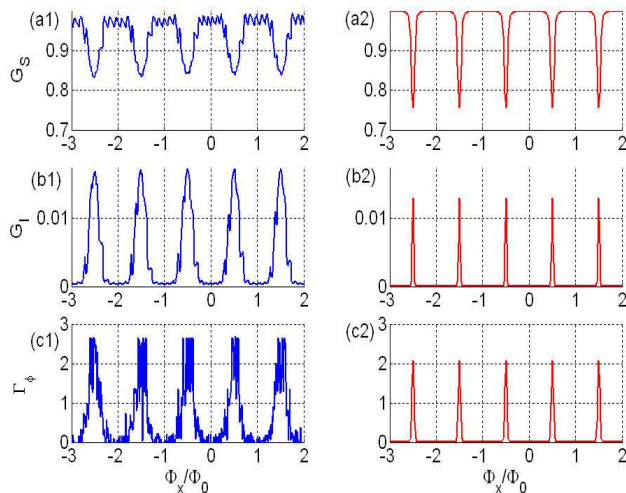
FIG. 5: (Color online) Signal gain G_s , idler gain G_i , and normalized dephasing rate \Gamma_\varphi . Experimental results are shown in panels (a1), (b1) and (c1), whereas theoretical predictions are shown in panels (a2), (b2) and (c2). The following device parameters were taken in order to evaluate G_s and G_i theoretically using Eqs. (82) and (83) of Ref. [24] [panels (a2) and (b2) respectively], and to evaluate \Gamma_\varphi using Eq. (70) of Ref. [8] [panel (c2)]: (\gamma_{f3} + \gamma_{d3})/\omega_1 = 5000 , \gamma_{f3}/\gamma_{d3} = 0.15 , I_{c1} = 1.5 \mu\text{A} and I_{c2} = 4.5 \mu\text{A} . Note that the effect of nonlinear damping [24] is disregarded.
