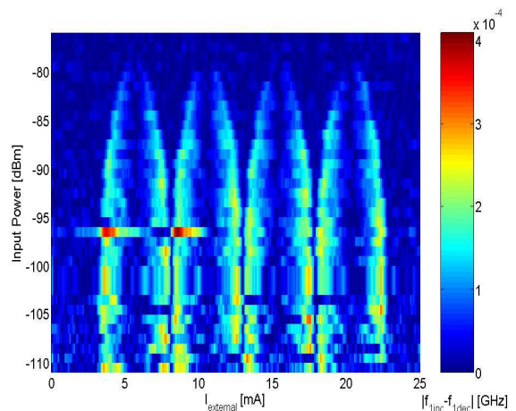
FIG. 7: The difference between the measured resonance frequencies obtained in the increasing flux sweep ( f_{1\text{inc}} ) and the decreasing flux sweep ( f_{1\text{dec}} ) of the first ( detector ) mode. The dark blue areas correspond to monostable regions, namely, the same resonance frequency is measured for both the increased and decreased sweep. The red indicates the regions where the system is bistable.
