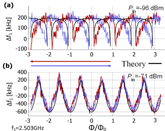
FIG. 3: (Color online) The resonance frequency shift \Delta f_1 of the first (detector) mode vs. applied flux for two different values of P_{\text{in}} . The flux is first swept upwards (blue line) and then downwards (red line). The black solid lines represent the theoretical calculation of \Delta f_1 using the following parameters: \beta_L = 7.4 for P_{\text{in}} = -96 dBm, \beta_L = 0.15 for P_{\text{in}} = -71 dBm, and I_{c1}/I_{c2} = 3 for both cases.
