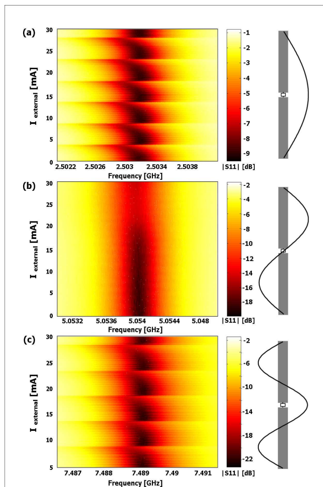
FIG. 2: (Color online) Reflection coefficient |S_{11}| vs. frequency and external flux for the first 3 modes of the SSR. A change of 4.8 mA in the external current corresponds to a change of \Phi_0 in the magnetic flux.
