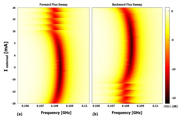
FIG. 6: Measured |S_{11}| at input power P_{\text{in}} = -95\text{dBm} for forward (a) and backward (b) magnetic flux sweep. In this sample \beta_L = 20 , and the response is highly hysteretic.
