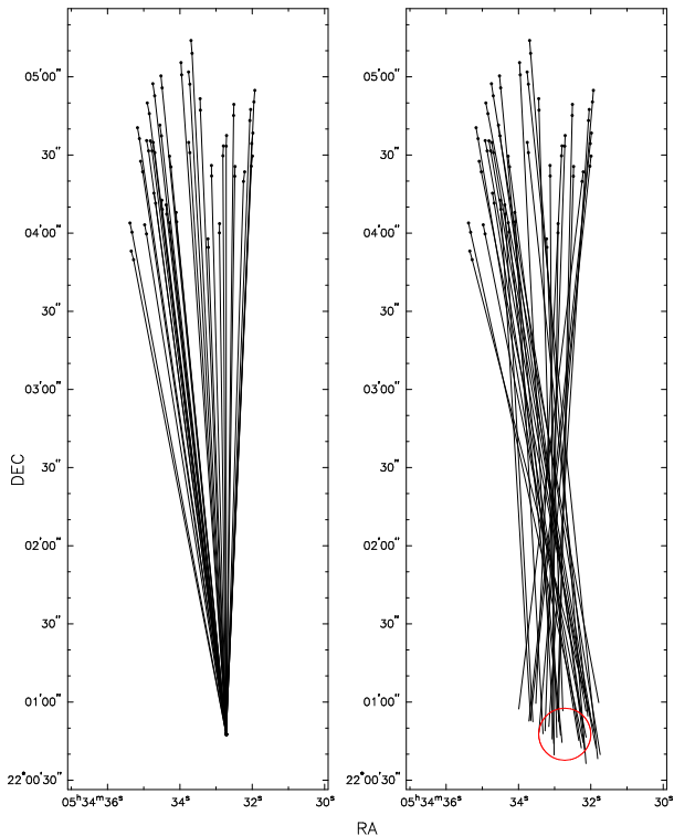
Figure 5. Plots of the extrapolated proper motions of the jet knots. Both plots show two points, the measured positions of the knots in 2005 and 1988. The lines in the left hand plot shows what the motions would look like if they were perfectly radial. The lines in the right hand plot show the true measured motions of the knots. The red circle is 10'' in radius centered on the center of expansion.
