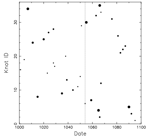
Figure 4. Plot of the computed convergence date of each knot upon the center of expansion. The size of the dot in the figure corresponds inversely to the distance between the traced back motion of the knot and the center of expansion. Thus the largest dots correspond to those knots which project back closest to the center of expansion.
