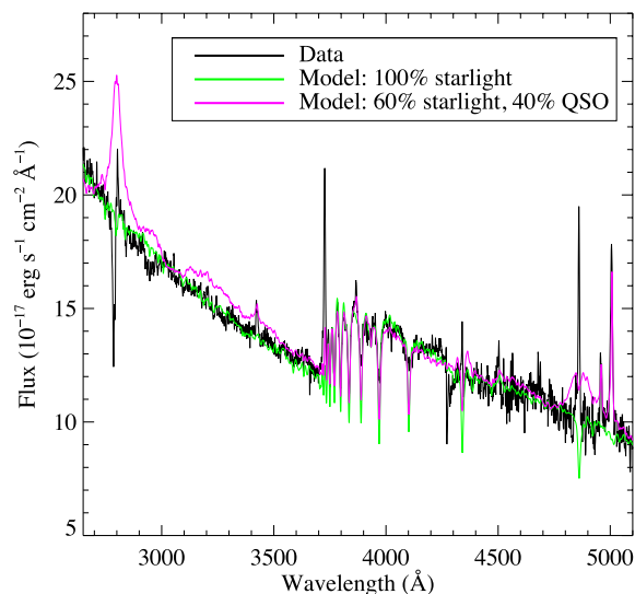
Figure 8. The black line shows the spectrum of J1506+54, a galaxy with an unresolved core that accounts for 47 per cent of the light in the rest-frame g -band HST image. The green line shows a stellar population model fit to the continuum. The magenta line shows a fit where a QSO template has been included. The QSO template accounts for 40 per cent of the light in the g band. The broad Mg II and H \beta emission lines are clearly visible in the template, but not in the data, ruling out the idea that the point source in the HST image is due to the presence of an unobscured AGN with a typical spectrum.
