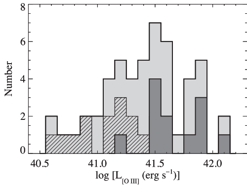
Figure 1. [\text{O III}] \lambda 5007 luminosities of the 51 galaxies with spectroscopic follow-up (light grey). Data that are upper limits are shown with hatched lines overlaid. The subsample of 12 galaxies studied here is shown in dark grey. These galaxies sample the upper half of the [\text{O III}] luminosity distribution.
