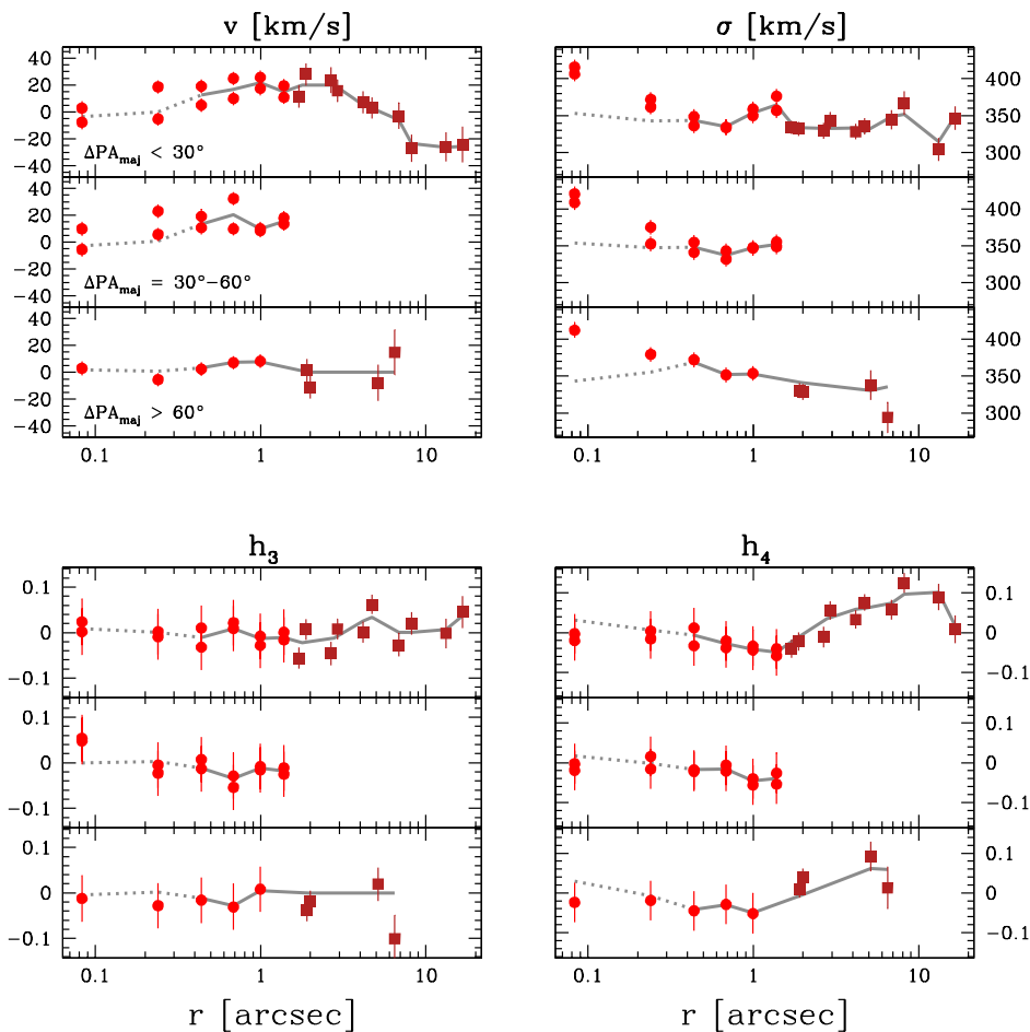
Figure 10. Kinematic data and the best-fit model. Points with error bars show the SINFONI (red circles) and SALT (dark-red squares) folded kinematic data – from top-left to bottom-right: rotation velocity v , dispersion \sigma , and Gauss-Hermite parameters h_3 and h_4 . Within each panel, data points are separated by the position angle ( \Delta\text{PA}_{\text{maj}} ) relative to the galaxy’s major axis. The grey solid lines indicate the best-fit dynamical model. Data points inside r < 0.35 arcsec were omitted in the fit (see Section 5). The dotted lines show the inward extrapolation of the dynamical model down to the smallest measured radius. Note that for the dynamical modelling we use the full LOSVDs (Section 5), which is essential for constraining the BH mass (see discussion in Appendix A).
