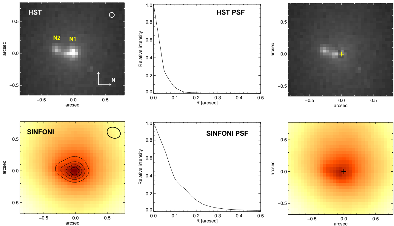
Figure 2. Close-up of the inner 1.5 \times 1.5 arcsec ( 410 \times 410 pc) of NGC 5419. Left panels: HST /WFPC2 F555W image and K -band VLT/SINFONI collapsed cube and isophotes. The images are centred at the position of the continuum maximum; the spatial orientation is indicated in the upper panel. N1 and N2 denote the central point source and the off-centre nucleus, respectively. The ellipses on the upper-right corners of the images indicate the Gaussian FWHM of the respective PSFs. Central and right panels show the corresponding PSF profiles and point-source subtracted images.
