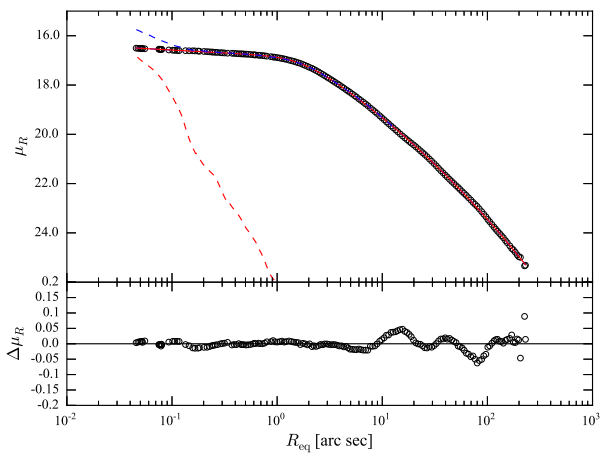
Figure 3. Surface brightness profile (circles), best-fitting Core-Sérsic model (red-solid line) and residuals. The blue- and red-dashed curves correspond to the HST surface brightness profile of NGC 5419 before the point source subtraction and the rescaled HST PSF profile, respectively (see Section 3.1 for details).
