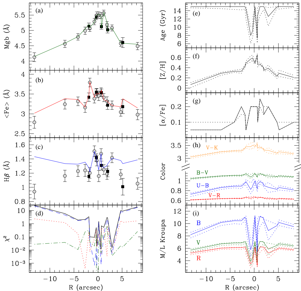
Figure 8. Panels (a)–(c): measured Lick indices profiles along the major (circles) and minor (squares) axes. The lines correspond to the best-fit single stellar population models. Panel (d): \chi^2 for each line index (the green dot-dashed line corresponds to Mg b, the red dotted line to Fe and the blue dashed line to H \beta ) and the total \chi^2 (black solid line). Panels (e)–(i): age, metallicity, overabundance, colours and M/L in different bands as a function of radius. The dotted lines show the 3\sigma errors.
