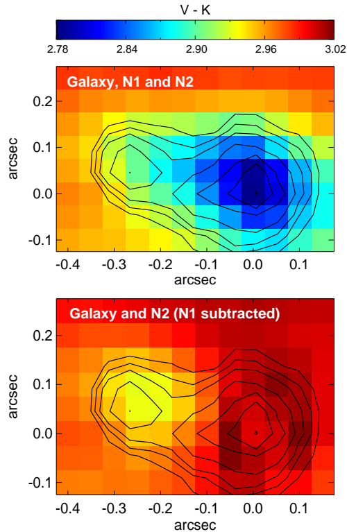
Figure 4. V-K colour maps derived from the HST and SINFONI images before (upper panel) and after (lower panel) the subtraction of the central point source. The contours correspond to the HST isophotes (see Fig. 2). North is right, east is up.
