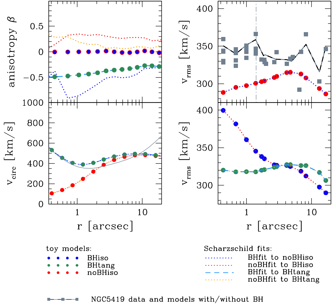
Figure A1. Anisotropy profiles (top-left panel), circular velocity curves (lower-left panel) and projected 2nd order moments v_{\text{rms}} (right panels). Dots show the values from the toy models while dotted and dashed lines show the fits to the model data. Also shown are the data (grey squares) and best-fitting Schwarzschild model with and without a BH obtained for NGC 5419 (solid grey and dashed black lines). The vertical dot-dashed line indicates the r_{501} estimated for NGC 5419's BH (see Section 5). BHiso, noBHiso and BHtang indicate the isotropic toy models with and without BH and the toy model with BH and tangential anisotropy, respectively. noBHfit and BHfit indicate the fits done assuming no BH and a M_{\text{BH}} = 7 \times 10^9 M_{\odot} , respectively. For the toy models and NGC 5419, fits with or without a BH do not produce noticeable differences in the 2nd order projected velocity moment.
