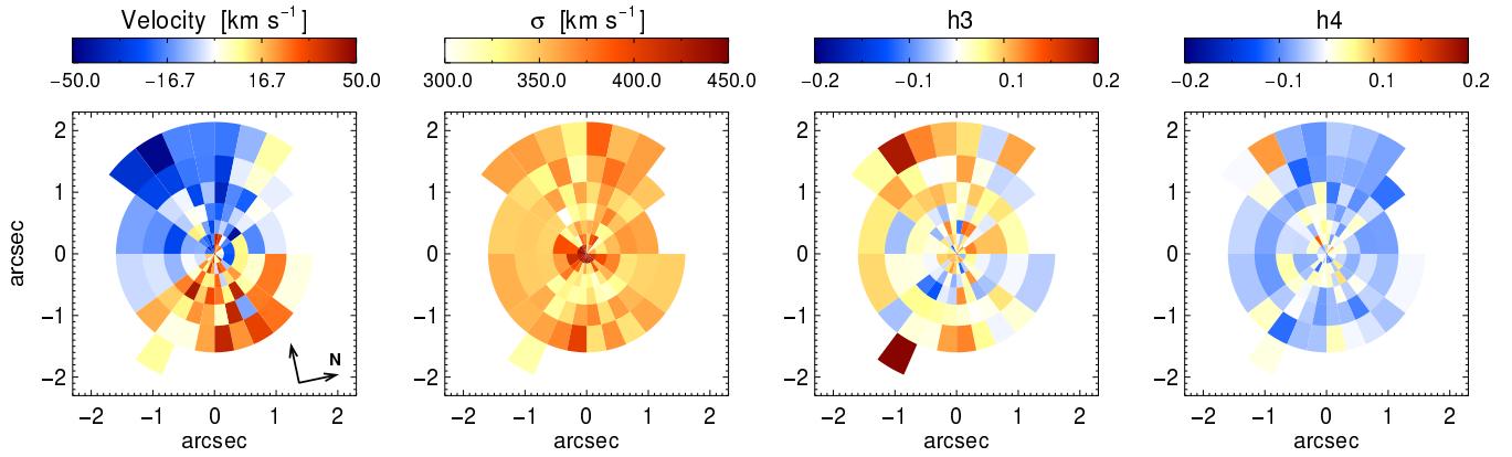
Figure 5. Kinematic maps of NGC 5419 derived from the SINFONI data. The spatial orientation is indicated in the left panel; the major axis of the galaxy is aligned with the y-axis.
