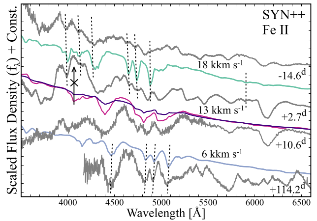
Figure 7. SYN++ single ion comparison for Fe II at 6000, 13 000, and 18 000 \text{km s}^{-1} . At post-maximum light phases (after day +10.6), Fe II overlaps nicely with the observed spectrum as a species formed near the photospheric line-forming region. At early epochs (day -14.6), high-velocity Fe II is a promising match. The arrow marked with \times signifies that contributions from Fe II are restricted by the data at this wavelength for the given v_{\min} .
