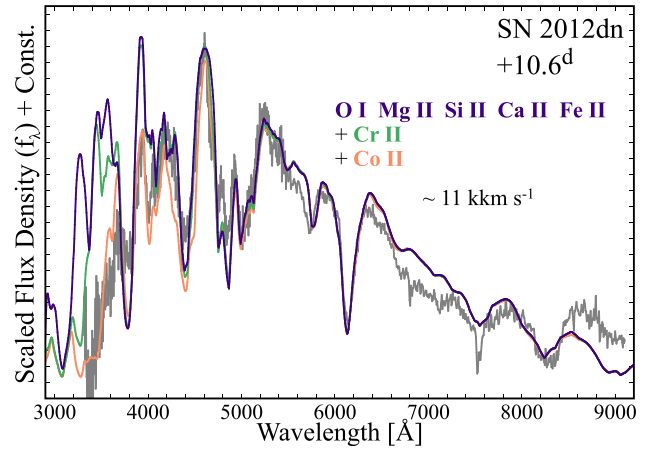
Figure 9. Composite synthetic spectra compared to the day +10.6 spectrum of SN 2012dn (in grey). Model v_{\min} are given in units of km s -1 1000 -1 . Na I has not been included in the fit, and forbidden lines of, e.g. Co III are not taken into account (see Childress et al. 2015).
